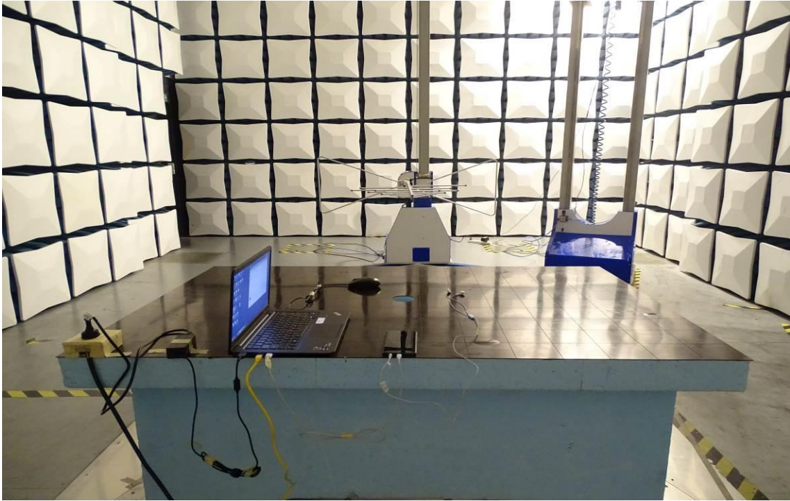
Radiated Disturbance Emissions (below 1GHz)
