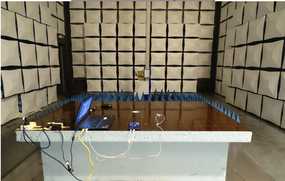
Radiated Disturbance Emissions (1GHz to18GHz)
