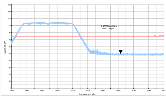
802.11b-Channel 11 Peak
