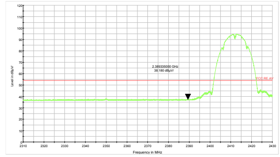
802.11b-Channel 1 Average
