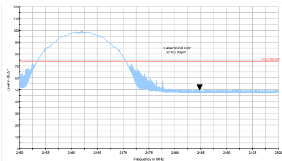
802.11g-Channel 11 Peak
