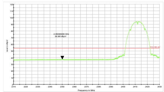
802.11g-Channel 1 Average
