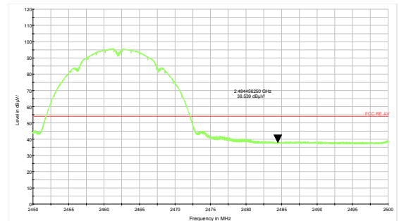
802.11g-Channel 11 Average
