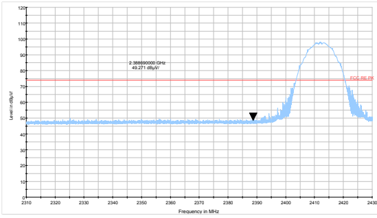
802.11b-Channel 1 Peak
