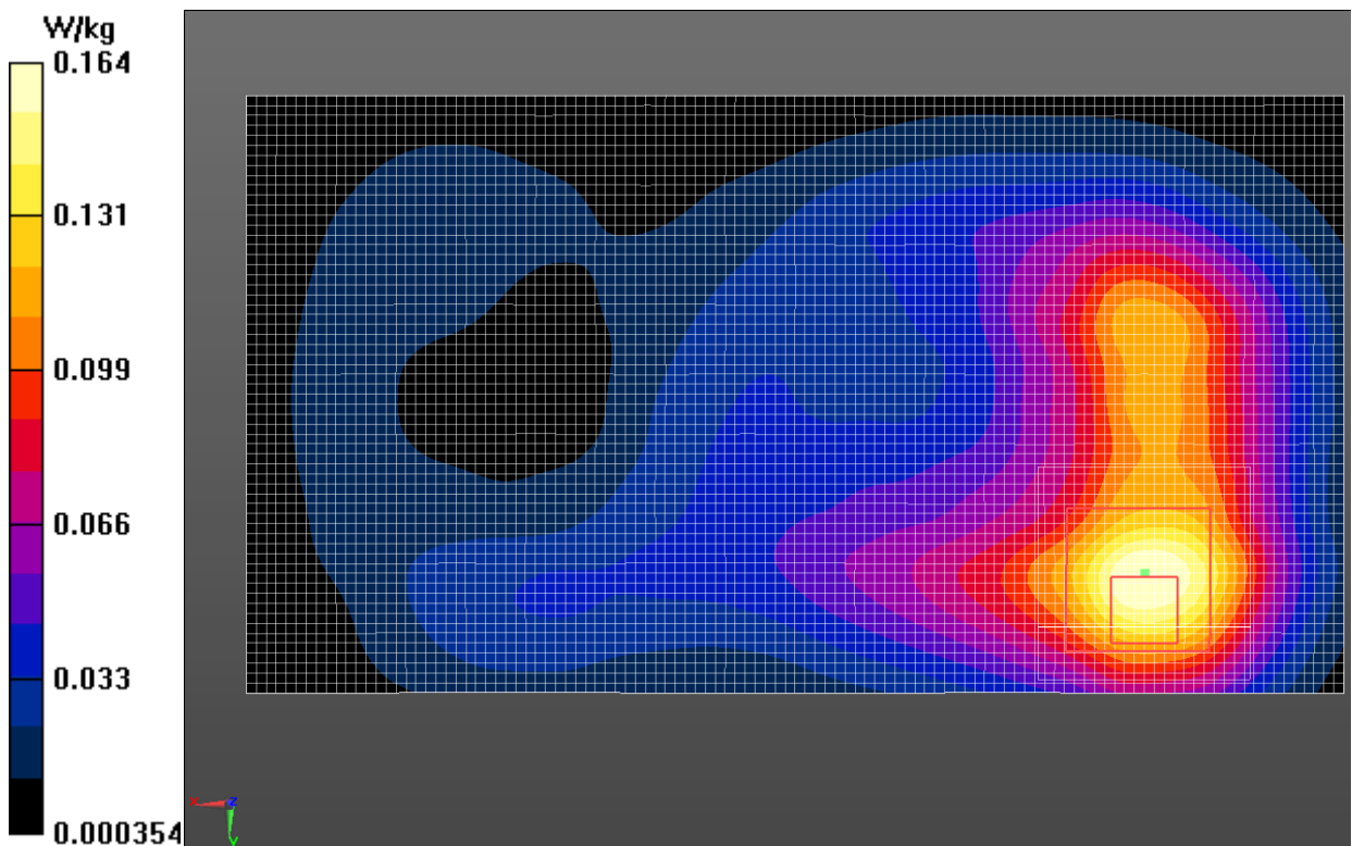
Fig.20 Wi-Fi 2.4G
