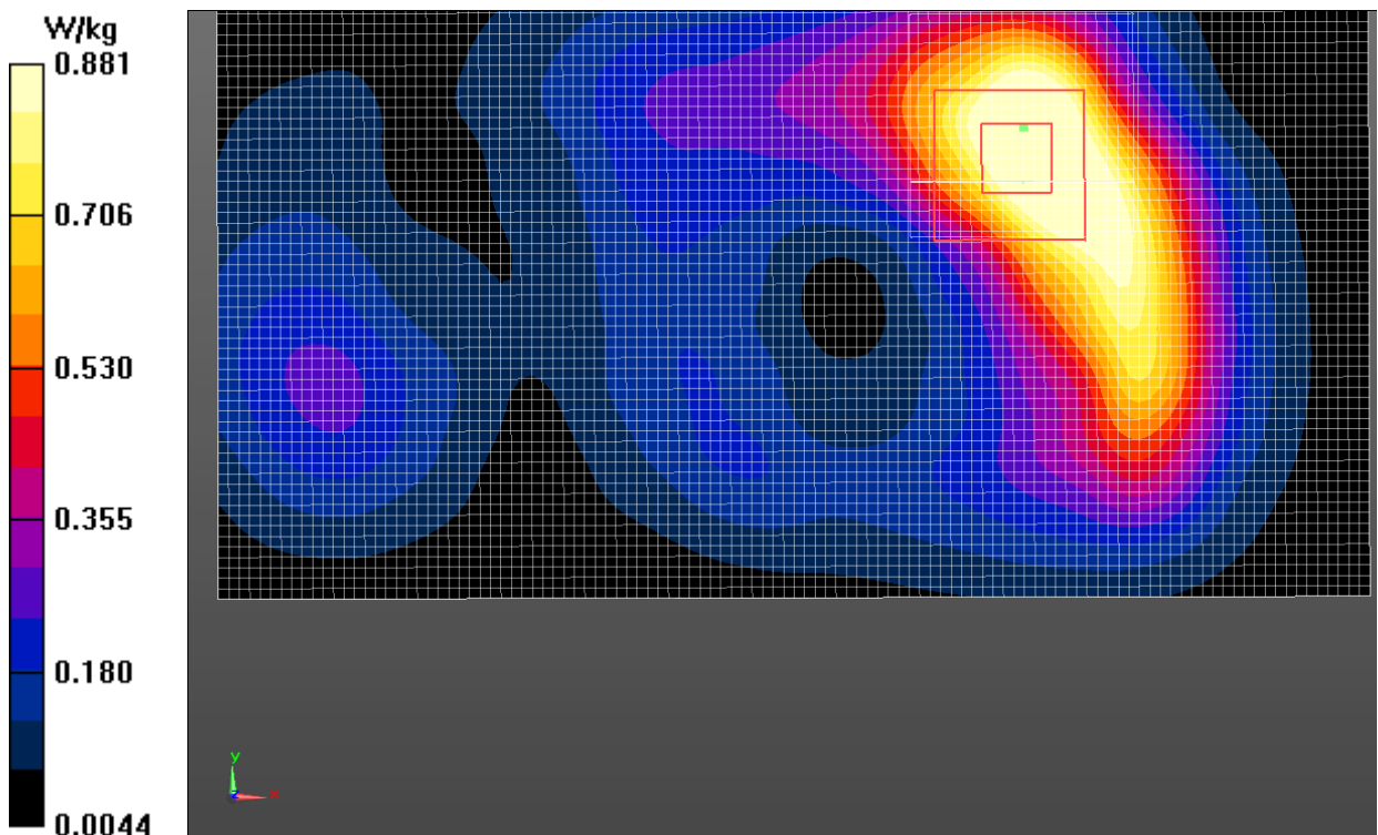
Fig.18 LTE Band 7
