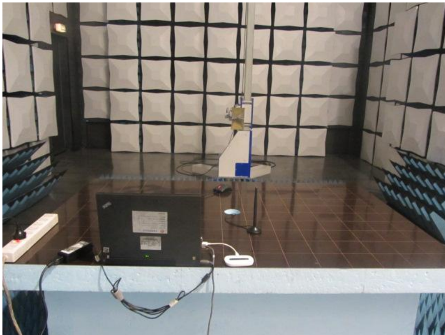
Radiated Disturbance (1GHz To 18GHz)
