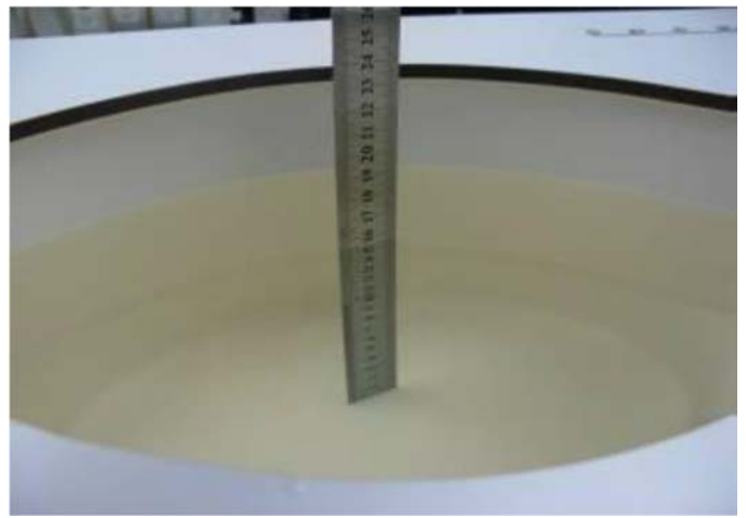
Photo 26: MSL2450MHz depth (15.1cm)
