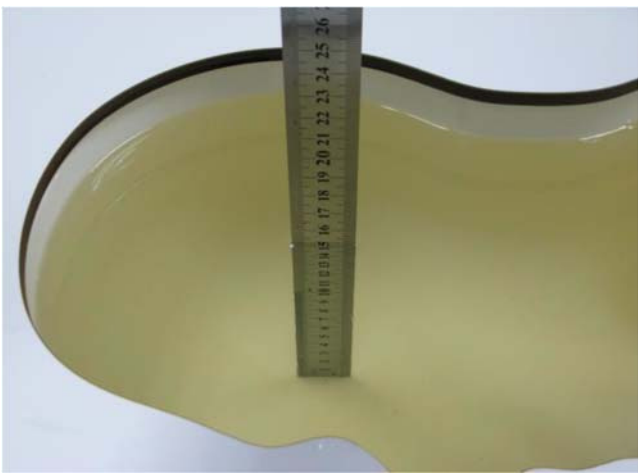
Photo 27: HSL2600MHz depth (15.0cm)
