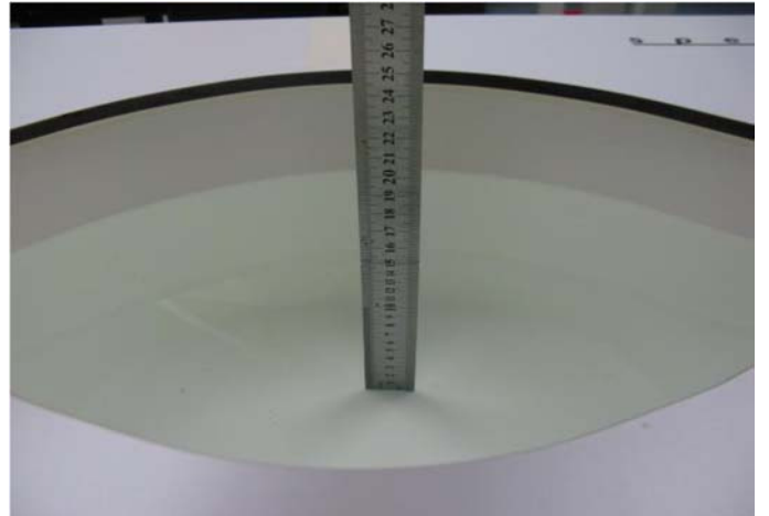
Photo 22: MSL1750MHz depth (15.1cm)
