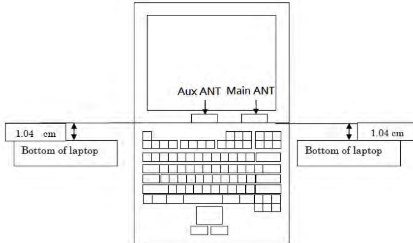
Fig.7 Antenna position of EUT (Front view)
