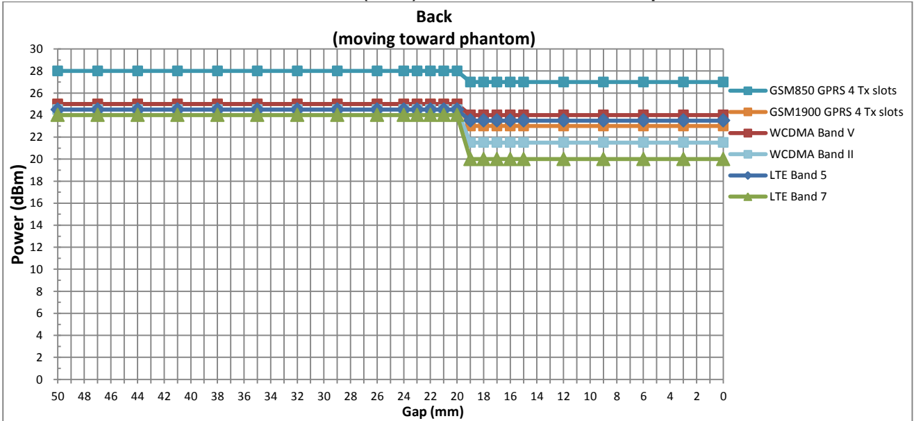
<The DUT (Back) is moved towards the flat phantom>
