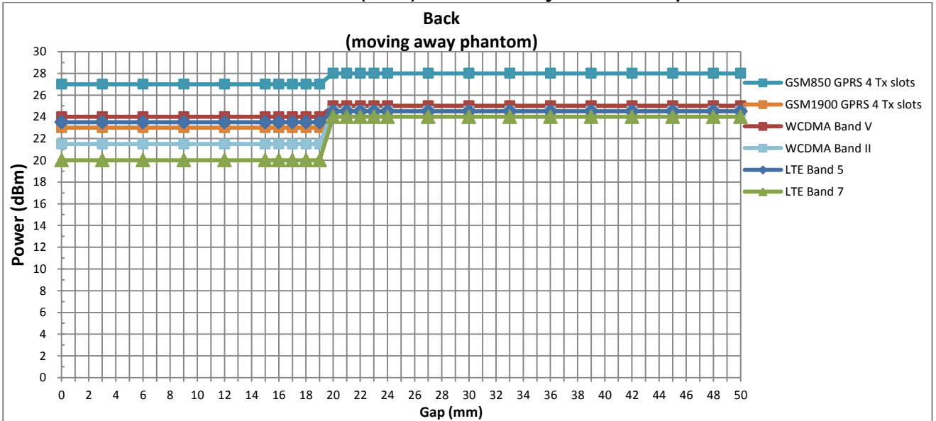
<The DUT (Back) is moved away from the flat phantom>
