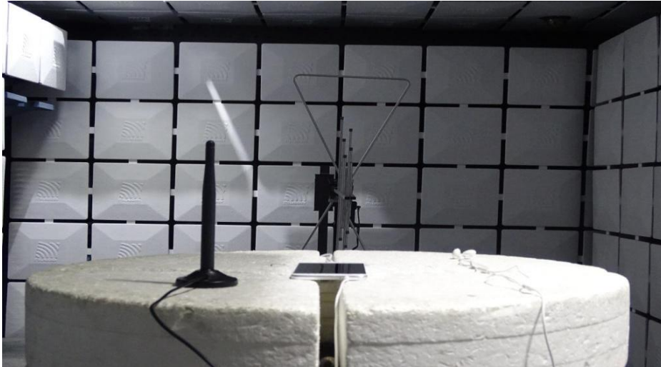
Radiated Spurious Emission (below 3GHz)
