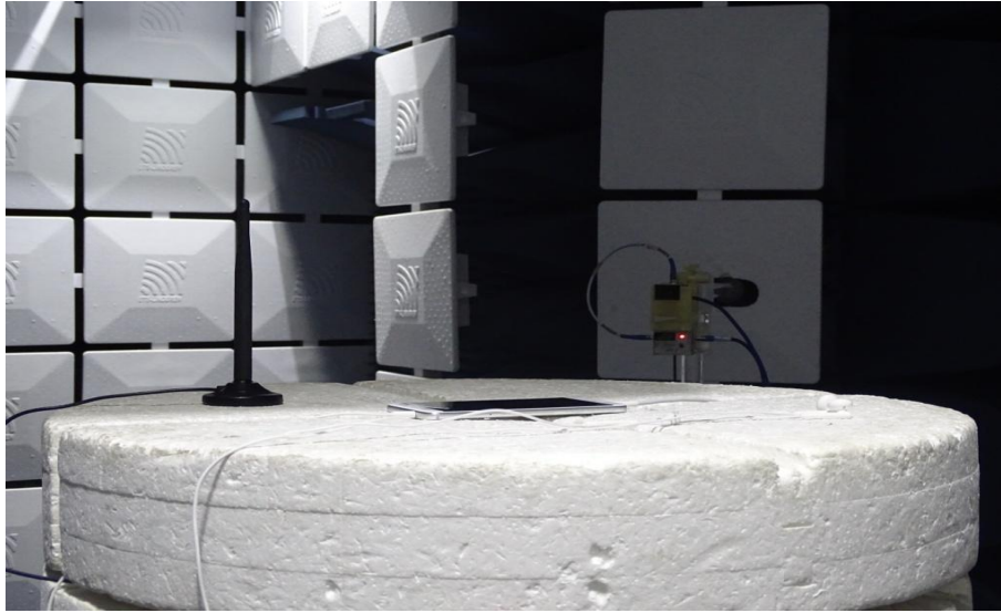
Radiated Spurious Emission (18GHz to26.5GHz)
