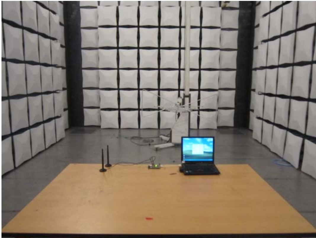
Photo 4 Radiated Disturbance Test (30MHz-1GHz)
