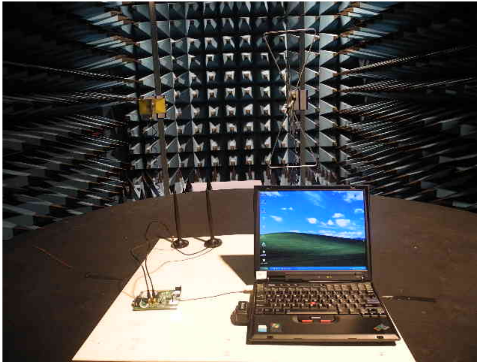
Photo 5 Radiated Disturbance Test (1GHz-6GHz)
