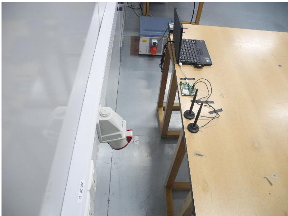
Photo 2 Conducted Disturbance Test
