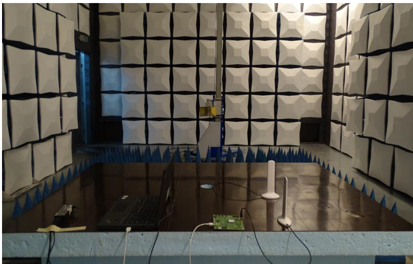
Radiated Disturbance Emissions (1GHz to 18GHz)
