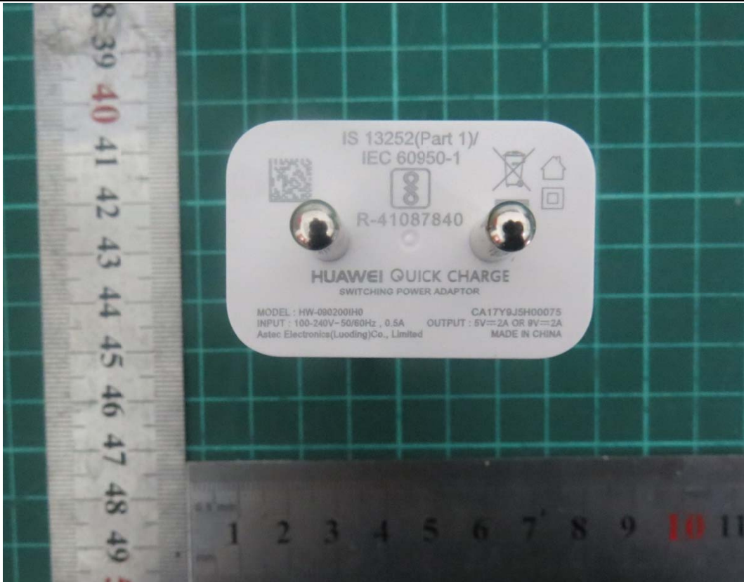
Adapter 7 b: Adapter
