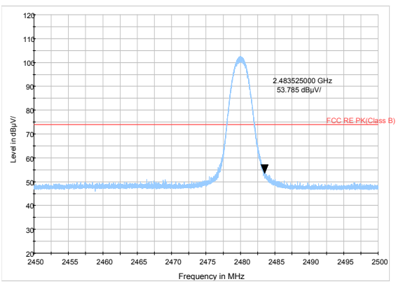
3DH5-Channel 78: Peak
