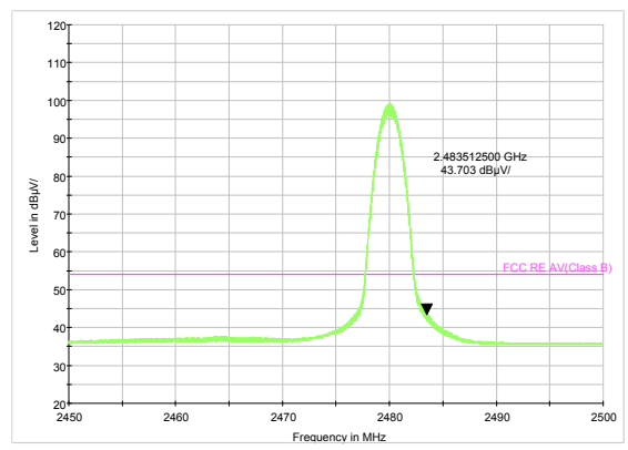
3DH5-Channel 78: Average
