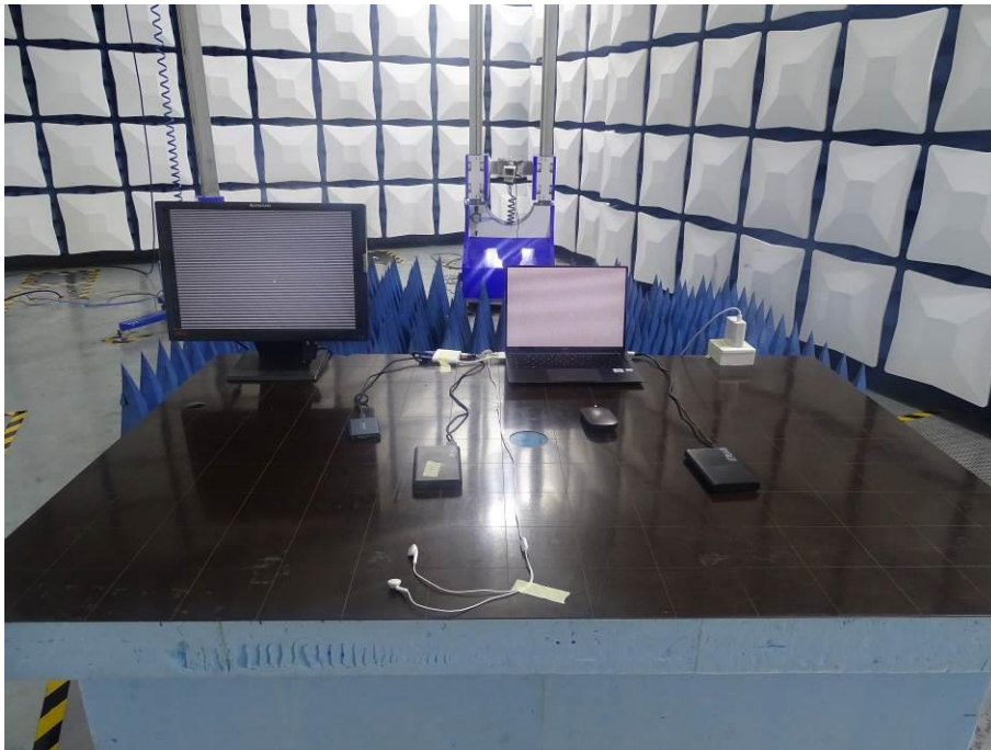
Radiated Disturbance Emissions (Above 18GHz)
