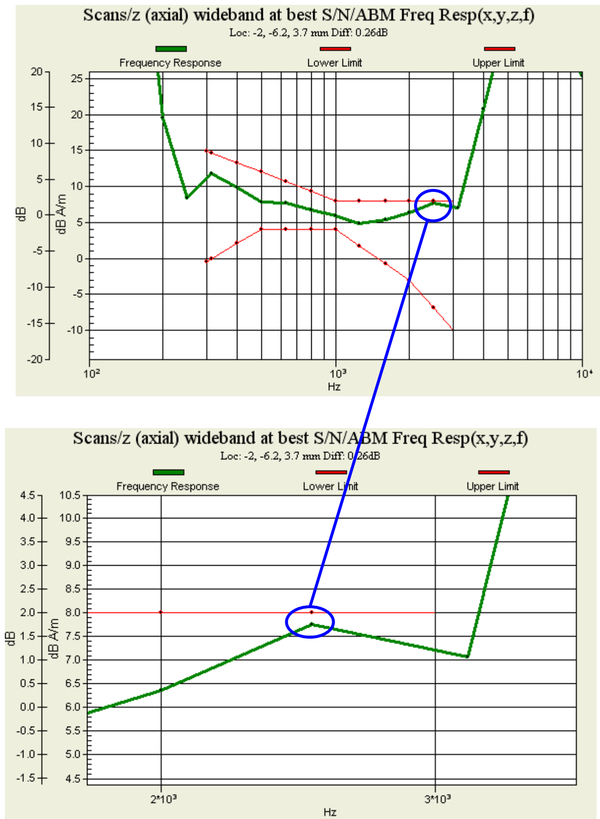
Figure 19 T-Coil CDMA AWS Z Axial
