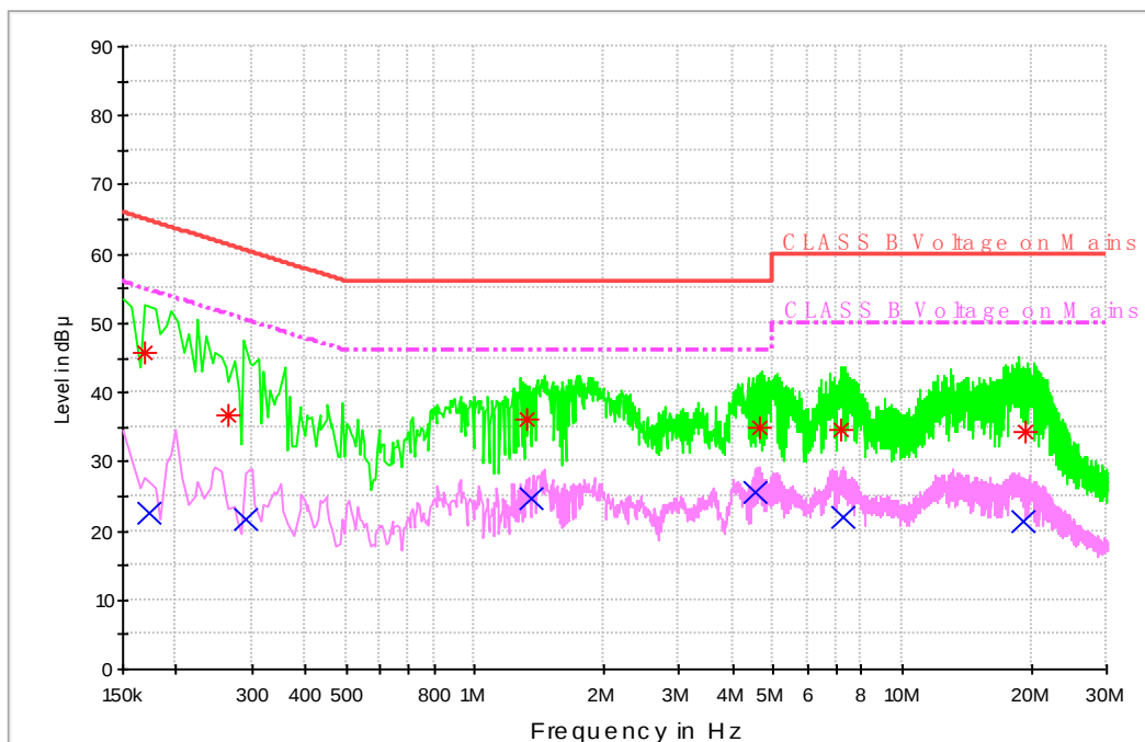
CLASS B Voltage with ENV216
