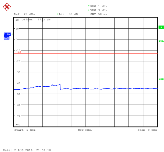
LTE Band 26 1.4MHz CH High 1GHz~9GHz
