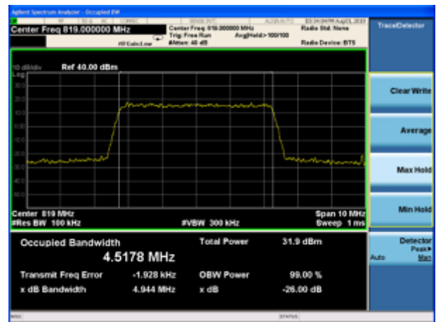
LTE Band 26 64QAM 5MHz CH Middle
