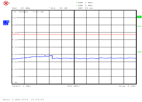
LTE Band 26 1.4MHz CH Low 1GHz~9GHz
