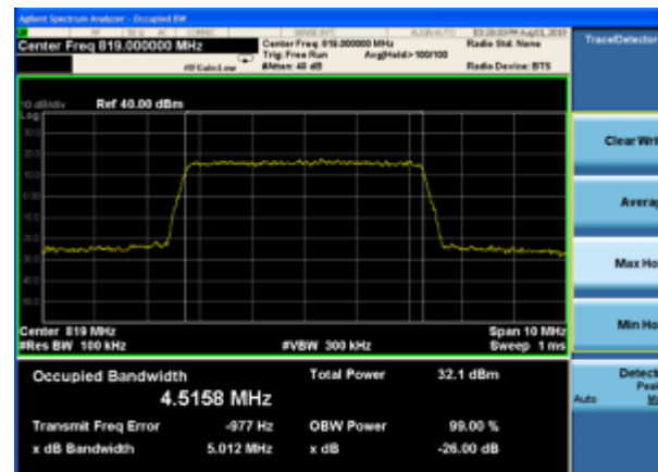
LTE Band 26 16QAM 5MHz CH Middle
