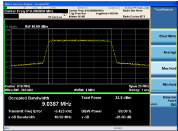
LTE Band 26 QPSK 10MHz CH Middle
