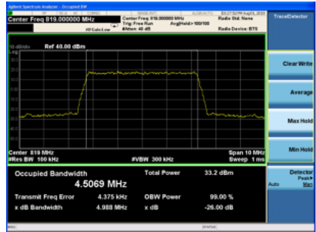
LTE Band 26 QPSK 5MHz CH Middle
