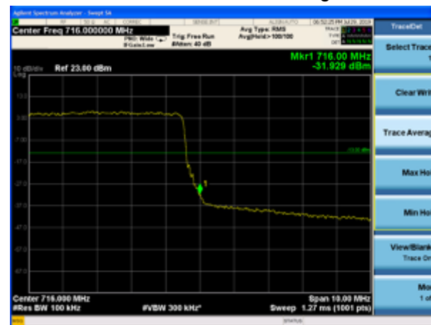
LTE Band 17 QPSK 10MHz CH-High, 100%RB
