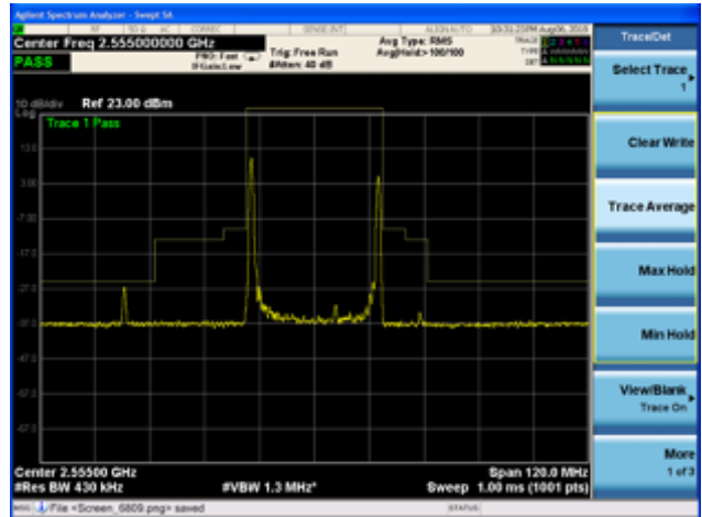
CA-7C 16QAM 20MHz+10MHz CH-High, 1 RB
