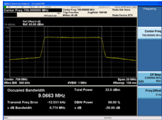
LTE Band 17 64QAM 10MHz CH-Middle
