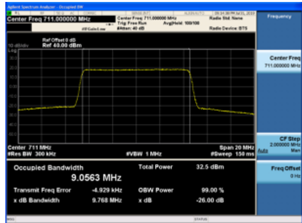
LTE Band 17 64QAM 10MHz CH-High
