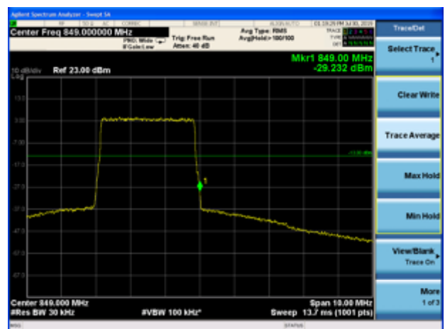
LTE Band 5 64QAM 3MHz CH-High 100%RB
