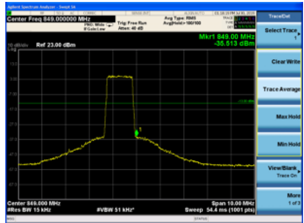
LTE Band 5 64QAM 3MHz CH-High 1RB
