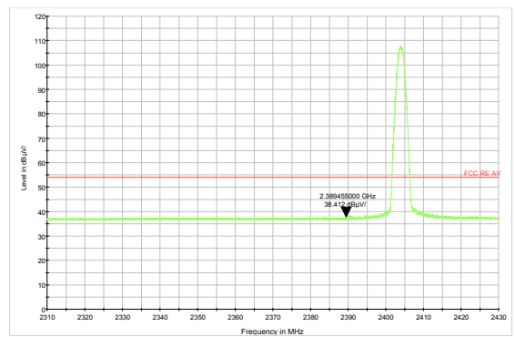
BT UHD BLE 1M GFSK 2404MHz: Average
