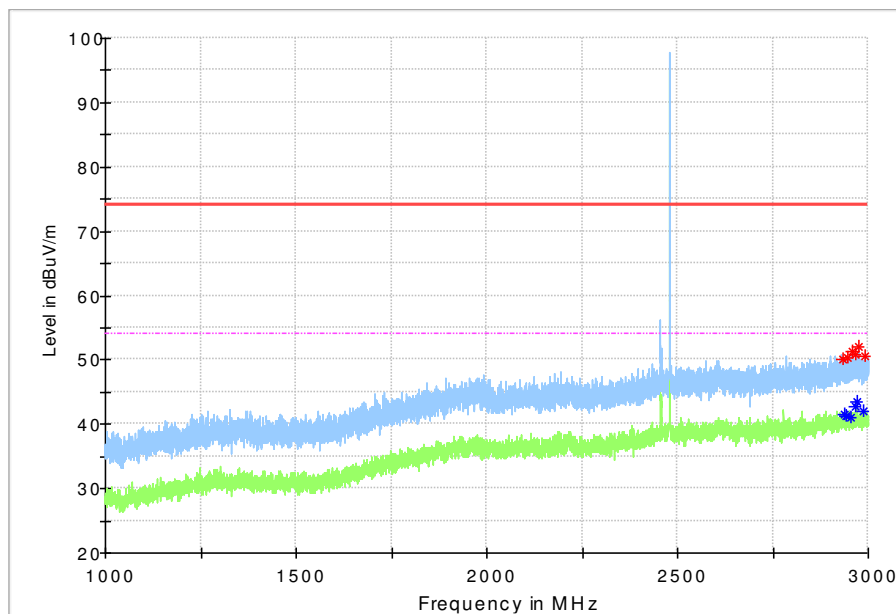
Fig. 68 Radiated Spurious Emission ( \pi/4 DQPSK, Ch78, 1 GHz ~3 GHz)
