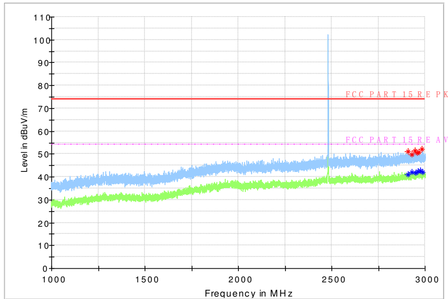
Fig. 79 Radiated Spurious Emission (8DPSK, Ch78, 1 GHz ~3 GHz)
