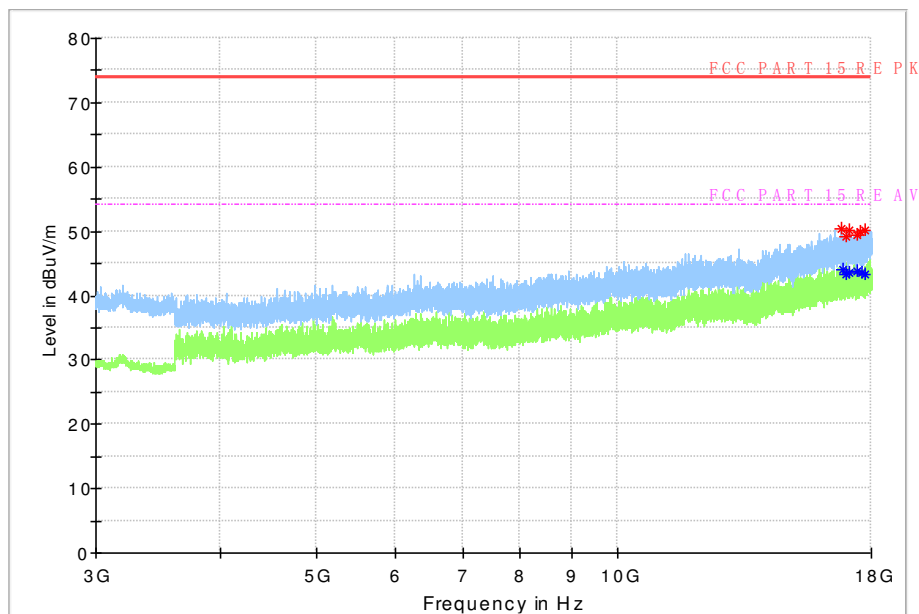
Fig. 66 Radiated Spurious Emission ( \pi/4 DQPSK, Ch39, 3 GHz ~18 GHz)
