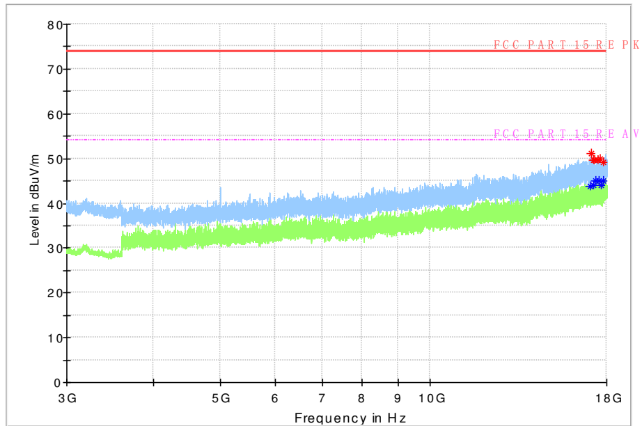
Fig. 69 Radiated Spurious Emission ( \pi/4 DQPSK, Ch78, 3 GHz ~18 GHz)
