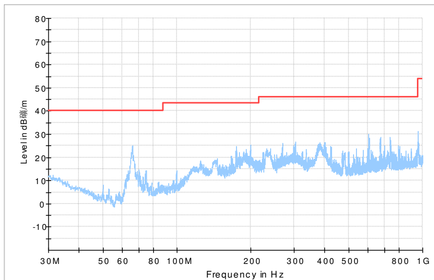
Fig. 64 Radiated Spurious Emission ( \pi/4 DQPSK, Ch39, 30 MHz ~1 GHz)
