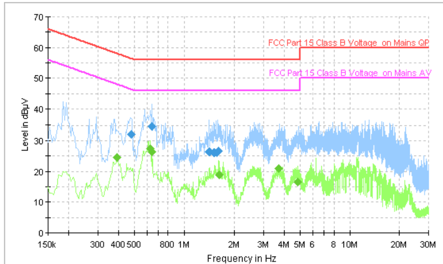
Fig. 117 AC Powerline Conducted Emission (Traffic, AE3)
