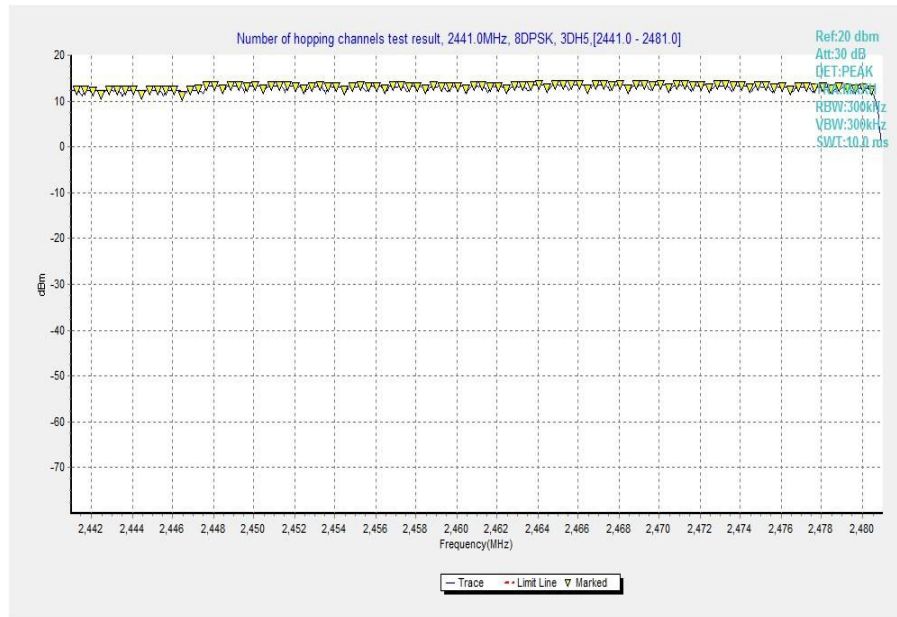
Fig. 103 Hopping channel ch39~78 (8DPSK, Ch39)
