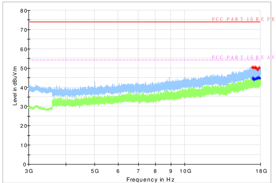
Fig. 77 Radiated Spurious Emission (8DPSK, Ch39, 3 GHz ~18 GHz)
