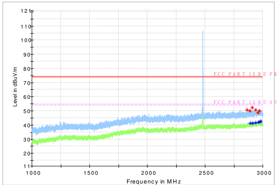
Fig. 57 Radiated Spurious Emission (GFSK, Ch78, 1 GHz ~3 GHz)
