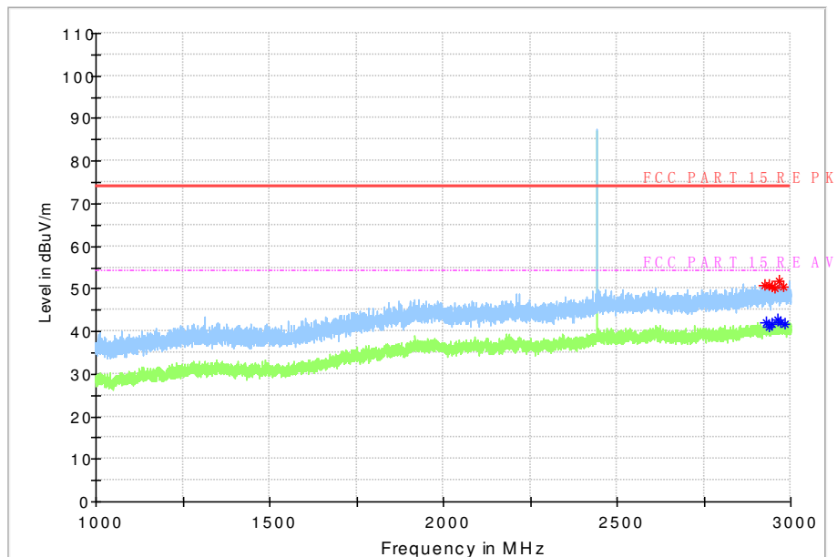
Fig. 76 Radiated Spurious Emission (8DPSK, Ch39, 1 GHz ~3 GHz)
