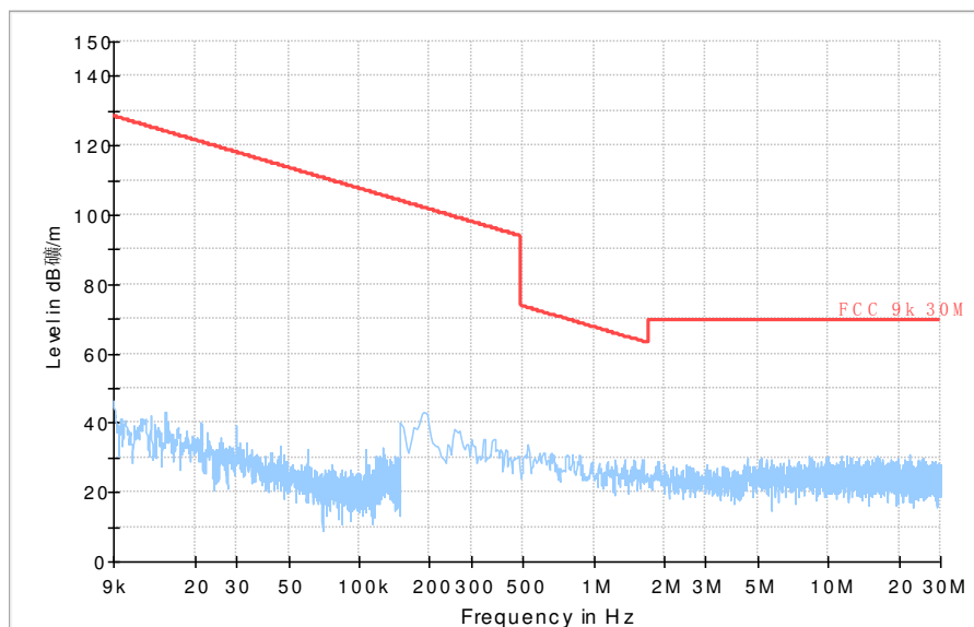
Fig. 74 Radiated Spurious Emission (8DPSK, Ch39, 9 kHz ~30 MHz)
