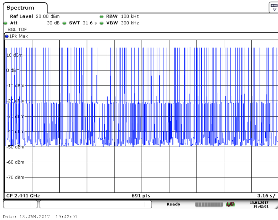
Fig. 93 Number of Transmissions (GFSK, Ch39)
