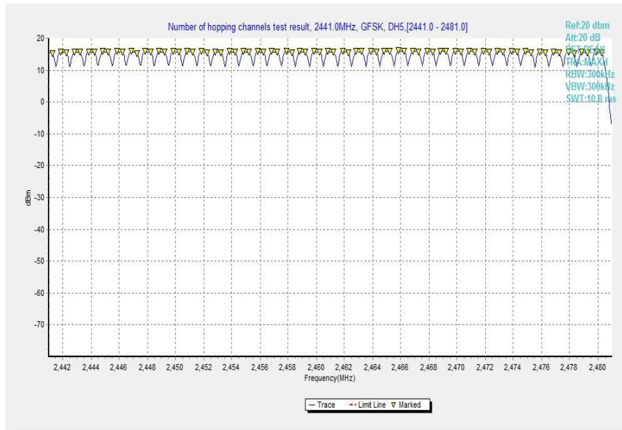
Fig. 99 Hopping channel ch39~78 (GFSK, Ch39)
