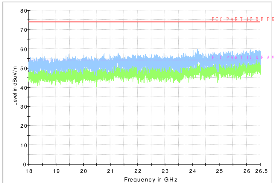
Fig. 67 Radiated Spurious Emission ( \pi/4 DQPSK, Ch39, 18 GHz ~26.5 GHz)
