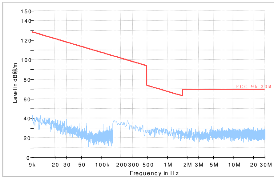
Fig. 63 Radiated Spurious Emission ( \pi/4 DQPSK, Ch39, 9 kHz ~30 MHz)
