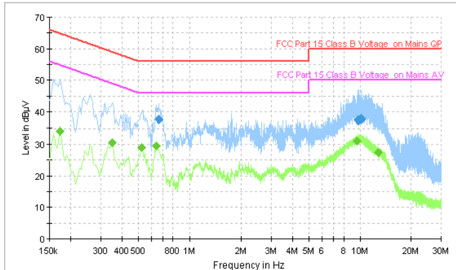
Fig. 114 AC Power line Conducted Emission (Idle, AE1)
