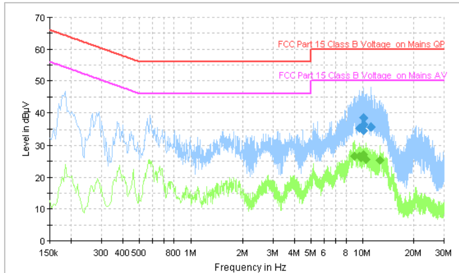
Fig. 113 AC Powerline Conducted Emission (Traffic, AE1)
