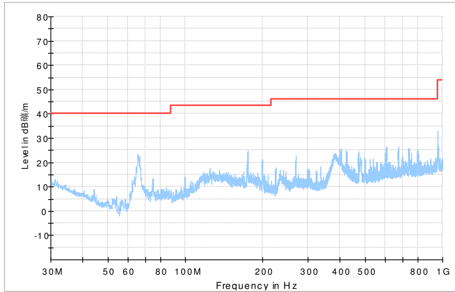
Fig. 75 Radiated Spurious Emission (8DPSK, Ch39, 30 MHz ~1 GHz)
