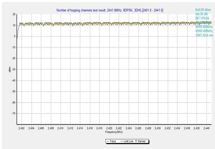
Fig. 102 Hopping channel ch0~39 (8DPSK, Ch39)
