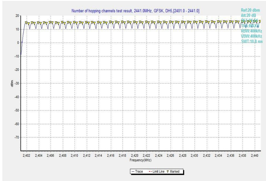
Fig. 98 Hopping channel ch0~39 (GFSK, Ch39)
