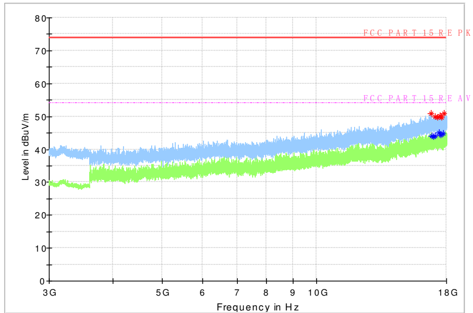
Fig. 73 Radiated Spurious Emission (8DPSK, Ch0, 3 GHz ~18 GHz)
