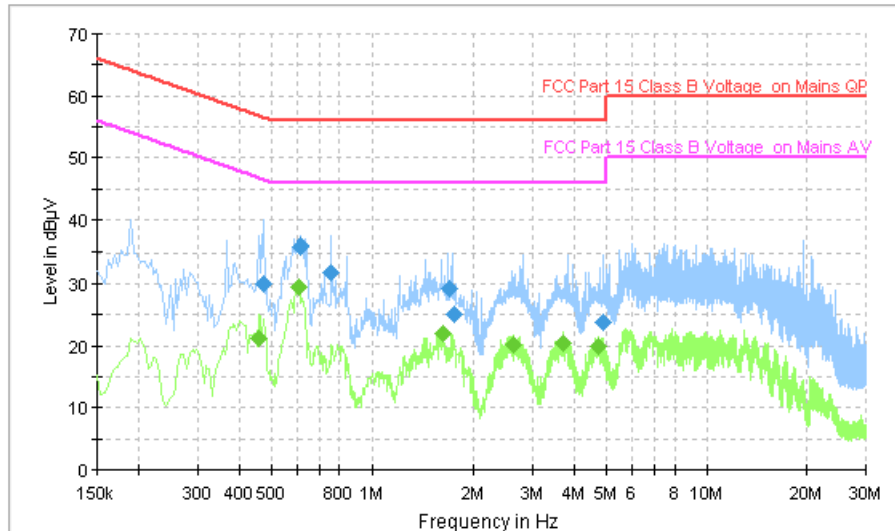
Fig. 112 AC Power line Conducted Emission (Idle, AE3)
