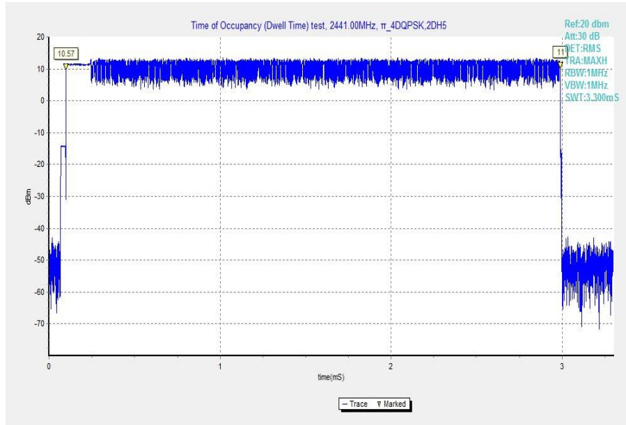
Fig. 94 Time of Occupancy(Dwell Time) ( \pi/4 DQPSK, Ch39)
