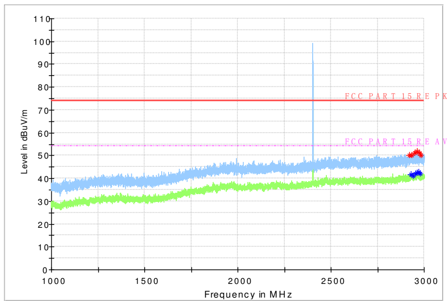
Fig. 72 Radiated Spurious Emission (8DPSK, Ch0, 1 GHz ~3 GHz)
