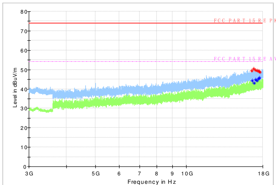
Fig. 80 Radiated Spurious Emission (8DPSK, Ch78, 3 GHz ~18 GHz)
