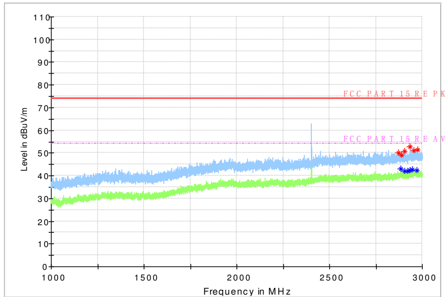
Fig. 61 Radiated Spurious Emission ( \pi/4 DQPSK, Ch0, 1 GHz ~3 GHz)
