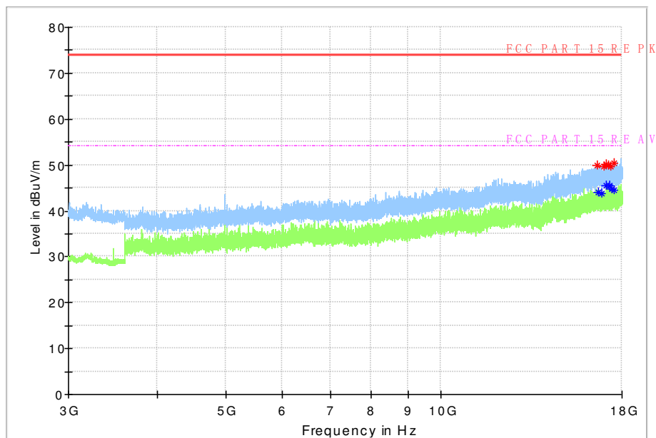
Fig. 62 Radiated Spurious Emission ( \pi/4 DQPSK, Ch0, 3 GHz ~18 GHz)
