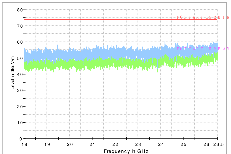
Fig. 78 Radiated Spurious Emission (8DPSK, Ch39, 18 GHz ~26.5 GHz)
