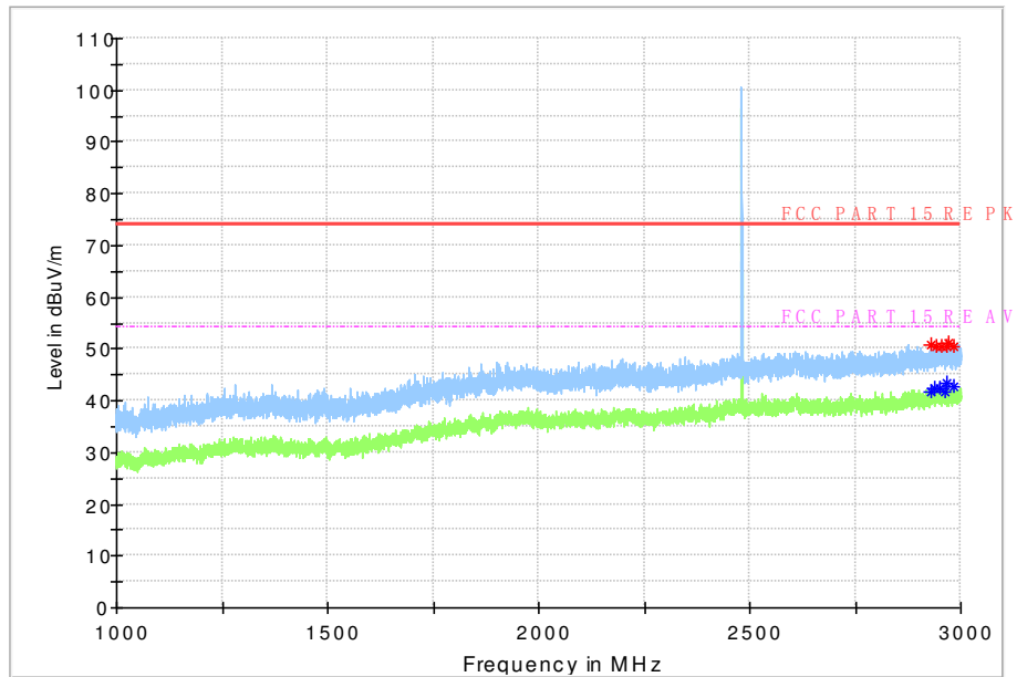
Fig. 65 Radiated Spurious Emission ( \pi/4 DQPSK, Ch39, 1 GHz ~3 GHz)
