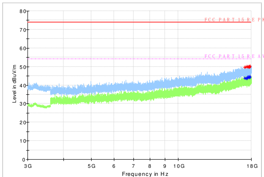
Fig. 58 Radiated Spurious Emission (GFSK, Ch78, 3 GHz ~18 GHz)
