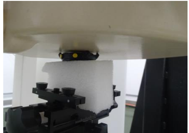
Photo 5: Back Side 0mm(LEO-BX9)
