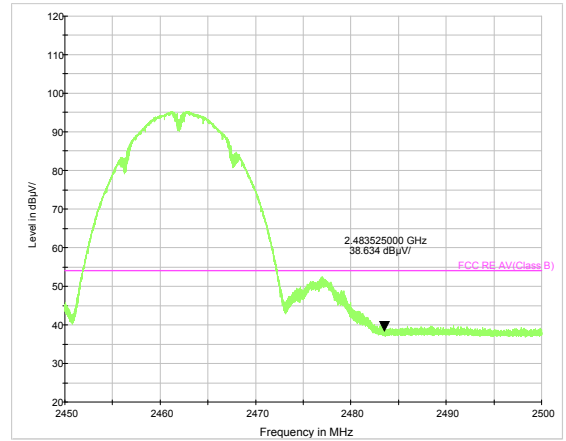
802.11b-Channel 11 Average
