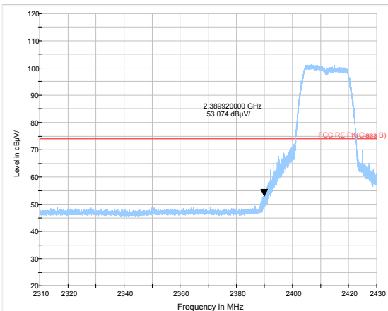
802.11g-Channel 1 Peak
