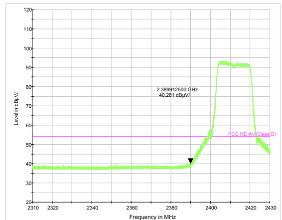
802.11g-Channel 1 Average
