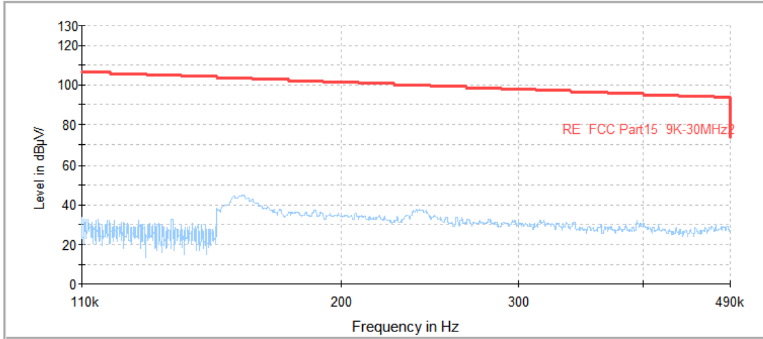
Radiates Emission from 110KHz to 490KHz
