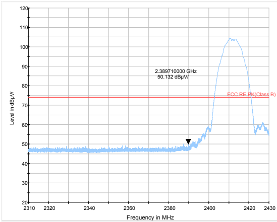
802.11b-Channel 1 Peak
