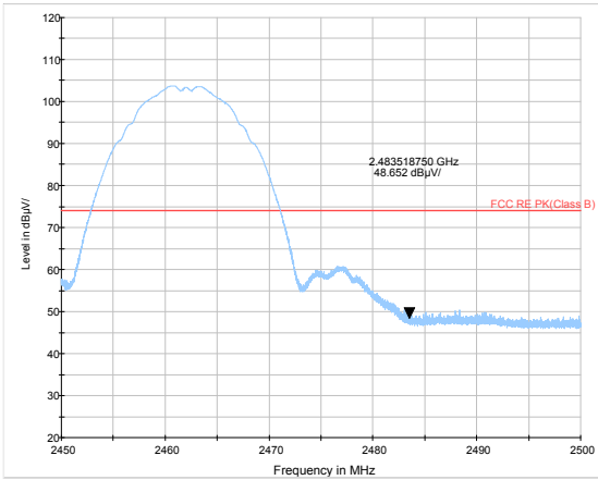
802.11b-Channel 11 Peak
