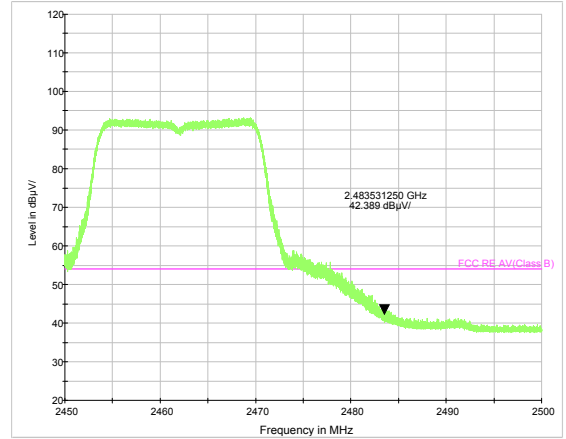
802.11g-Channel 11 Average
