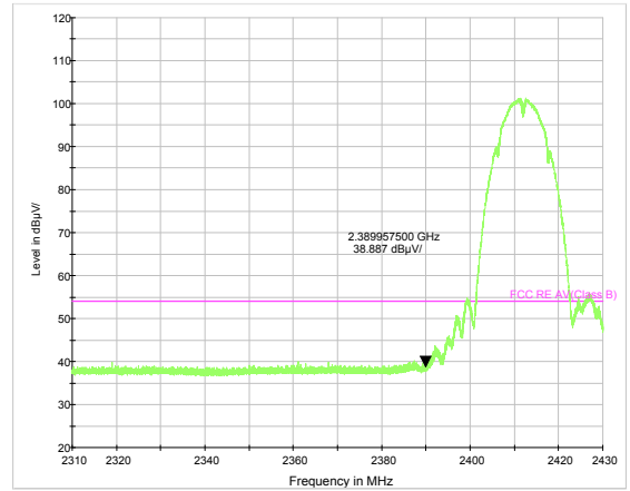
802.11b-Channel 1 Average
