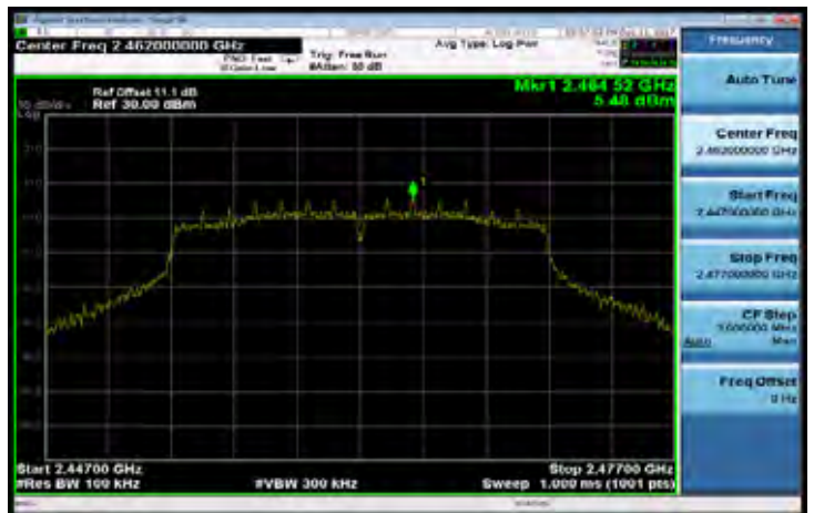
802.11n_HT20 Band Edge Limit Test Data CH-High
