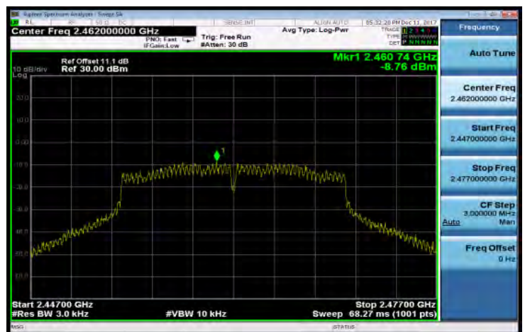
Power Spectral Density Test Plot (CH-High)
