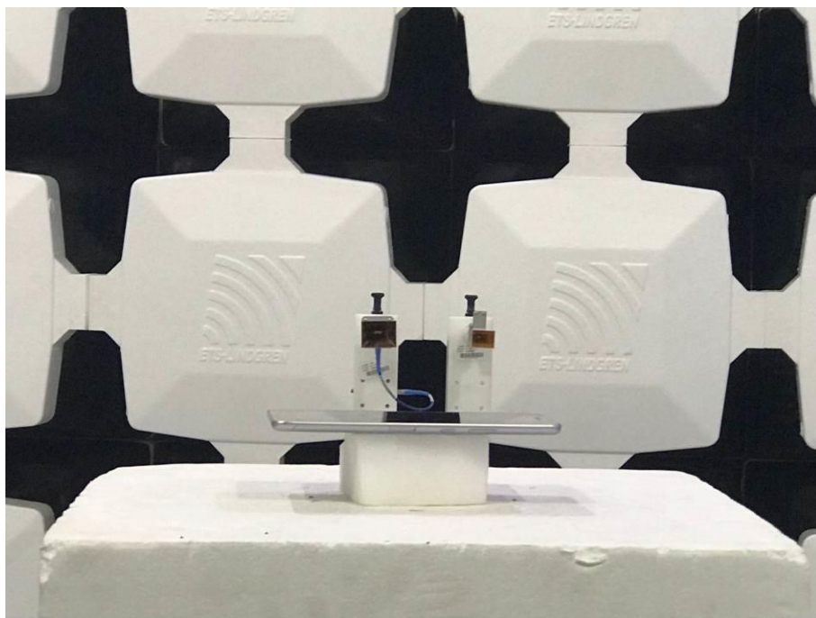
4. Radiated Emissions (Part 15 C&E) (18GHz-26.5GHz)
