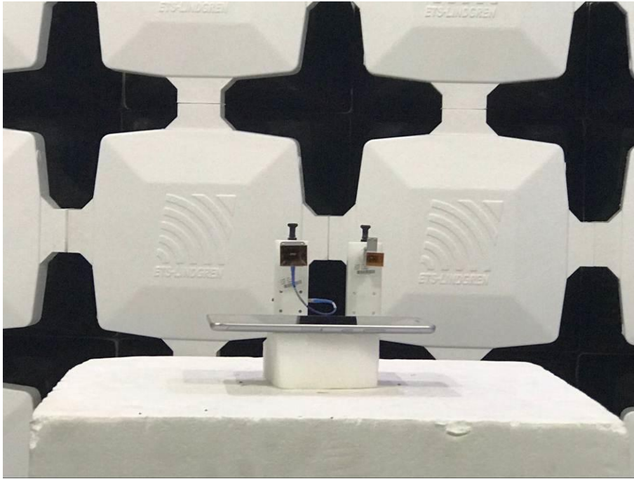
5. Radiated Emissions (Part 15 C&E) (26.5GHz-40GHz)
