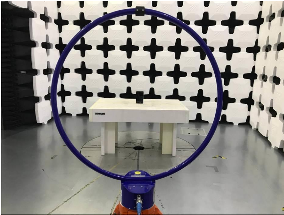
1. Radiated Emissions (Part 15C&E 9kHz-30MHz)
