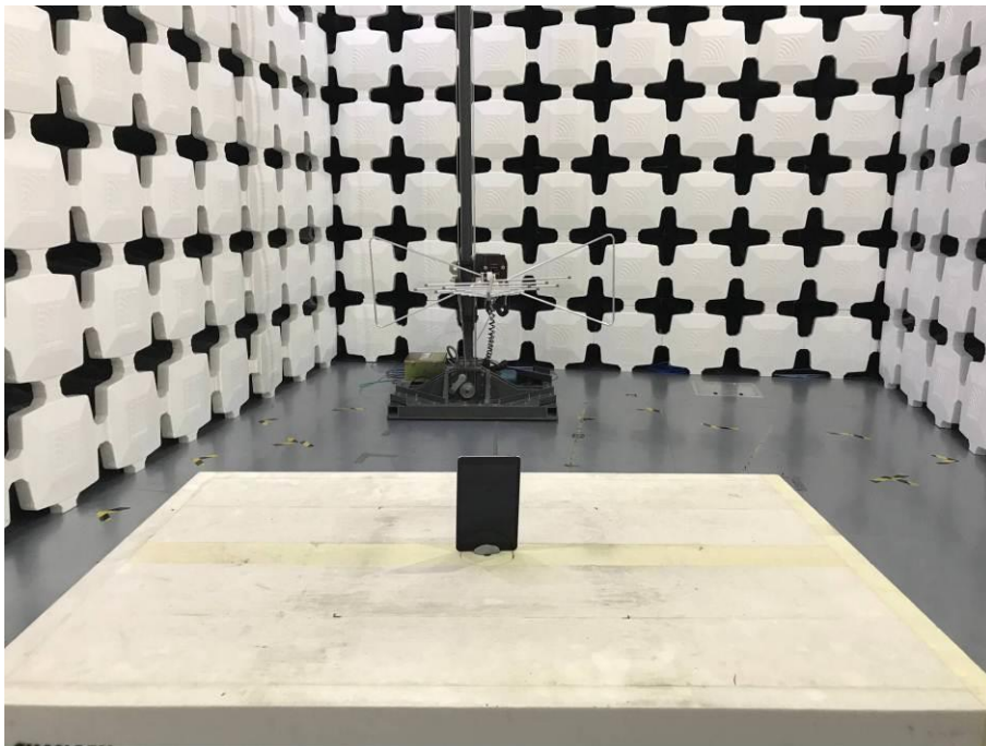
2. Radiated Emissions (Part 15 C&E 30M-1GHz)
