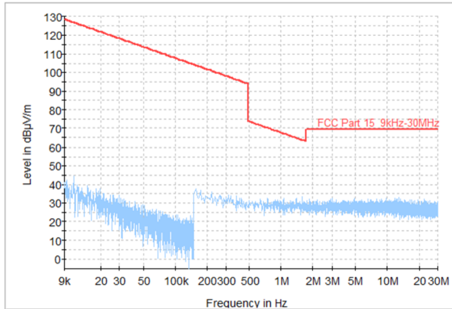
Fig. 1 Radiated Spurious Emission (8DPSK, Ch0, 9 kHz ~30 MHz)
