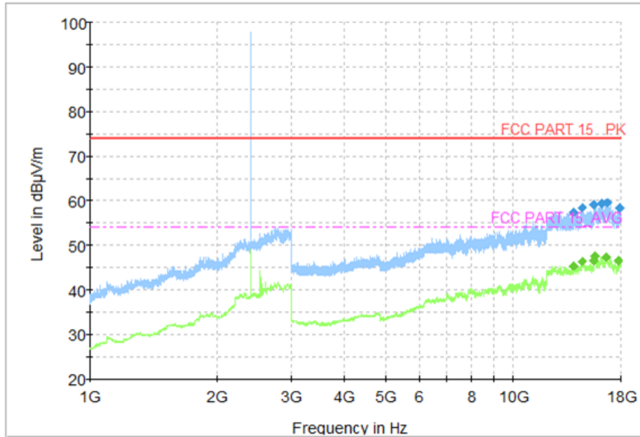
Fig. 3 Radiated Spurious Emission (8DPSK, Ch0, 1 GHz ~18 GHz)
