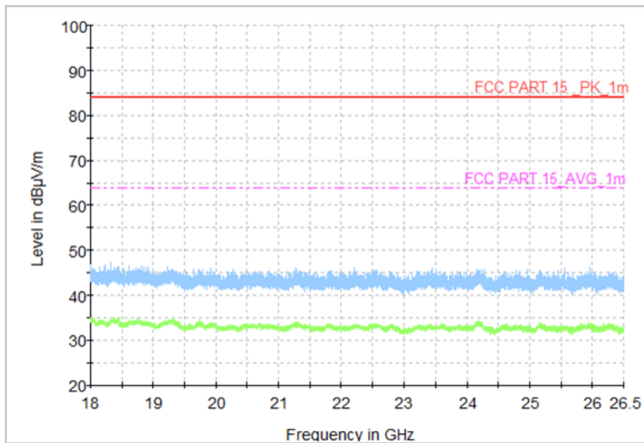
Fig. 4 Radiated Spurious Emission (8DPSK, Ch0, 18 GHz ~26.5 GHz)
