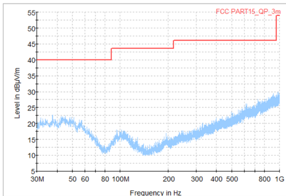
Fig. 2 Radiated Spurious Emission (8DPSK, Ch0, 30 MHz ~1 GHz)
