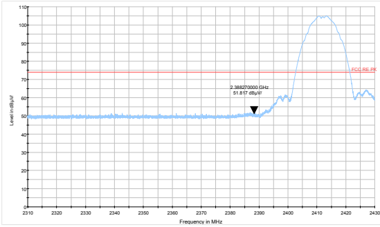
802.11b-Channel 1 Peak
