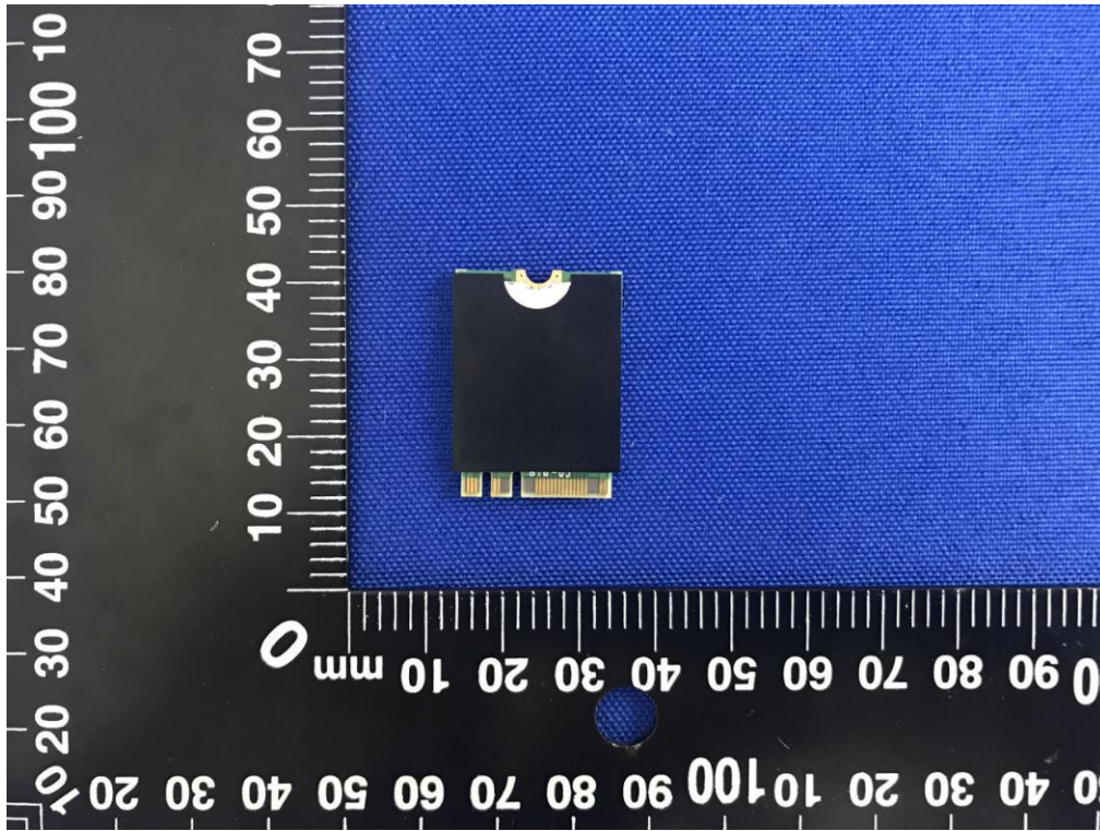
RF Module REAR VIEW (WITH SHIELDING)
