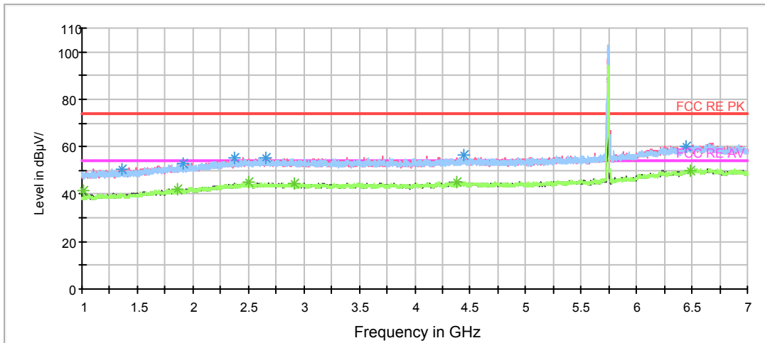
Note: The signal beyond the limit is carrier. Radiates Emission from 1GHz to 7GHz
