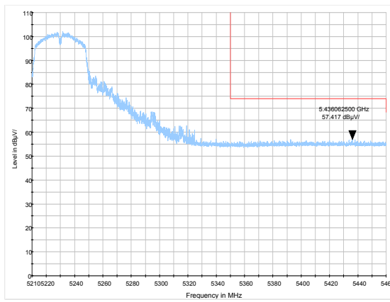
802.11n HT40-Channel 46: Average
