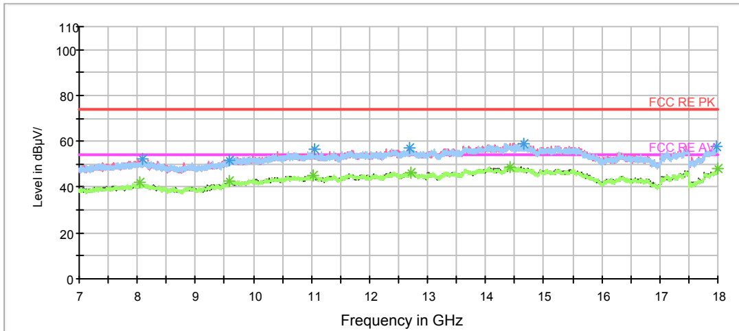
Radiates Emission from 7GHz to 18GHz
