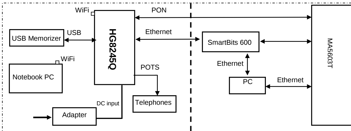
Figure 5. Test connection of TC1-TC2
