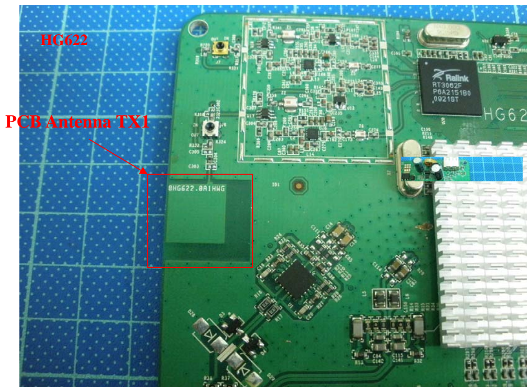
Photo 6: Internal photo of EUT
