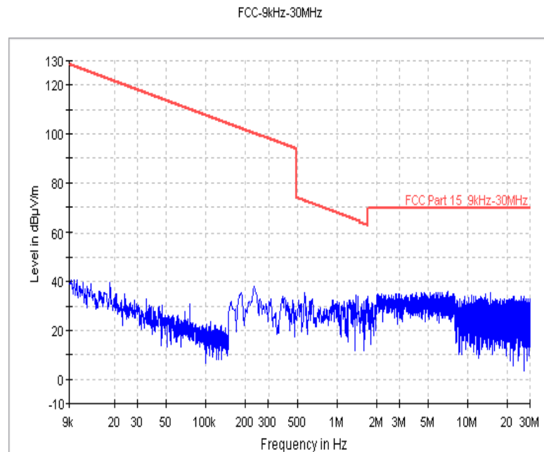
Fig.2 Radiated Spurious Emission (802.11b, Ch6, 9 kHz-30MHz)
