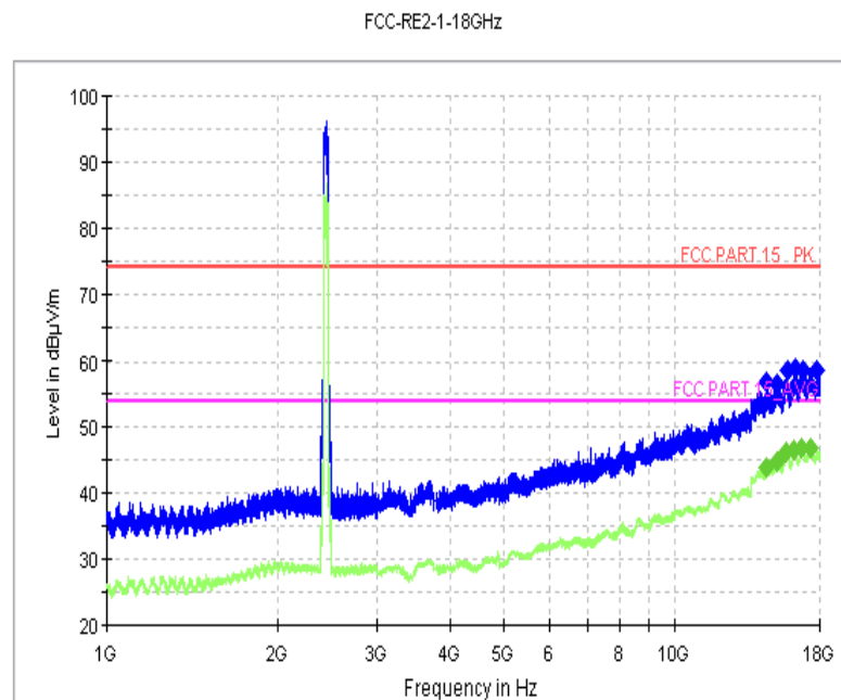
Fig.26 Radiated Spurious Emission (802.11 n-40MHz, Ch6, 1 GHz-18GHz)
