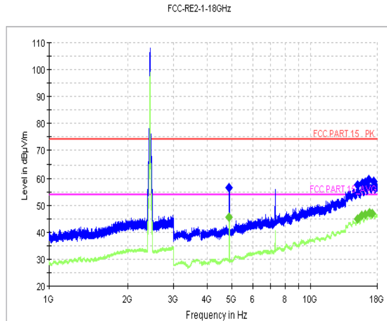
Fig.11 Radiated Spurious Emission (802.11g, Ch6, 1 GHz-18GHz)
