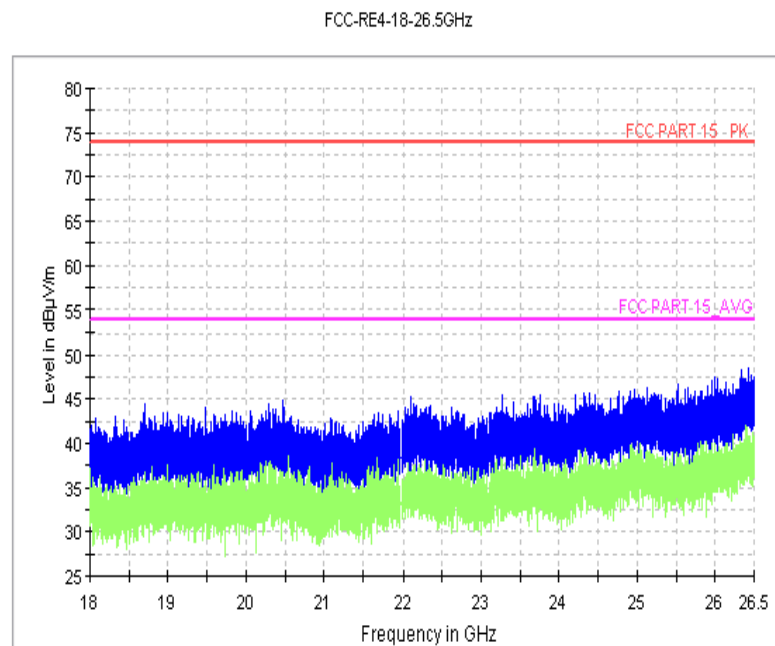
Fig.27 Radiated Spurious Emission (802.11 n-40MHz, Ch6, 18 GHz-26.5GHz)
