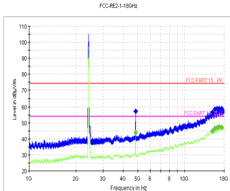
Fig.16 Radiated Spurious Emission (802.11n, Ch1, 1 GHz-18GHz)
