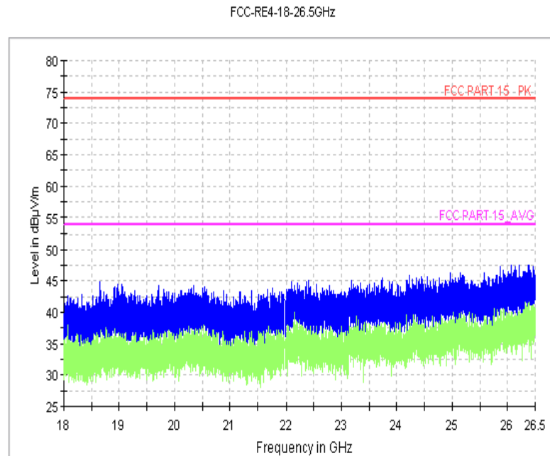
Fig.5 Radiated Spurious Emission (802.11b, Ch6, 18 GHz-26.5GHz)
