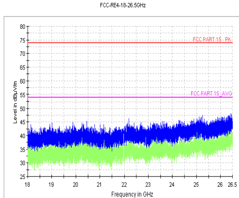
Fig.19 Radiated Spurious Emission (802.11n, Ch6, 18 GHz-26.5GHz)
