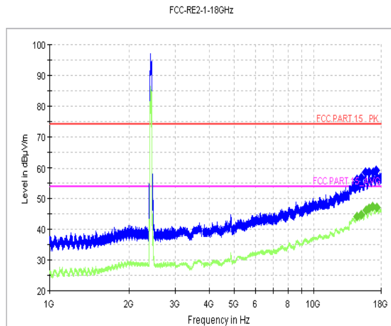
Fig.23 Radiated Spurious Emission (802.11n-40MHz, Ch3, 1 GHz-18GHz)
