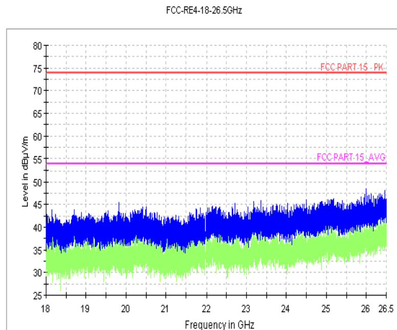
Fig.12 Radiated Spurious Emission (802.11g, Ch6, 18 GHz-26.5GHz)
