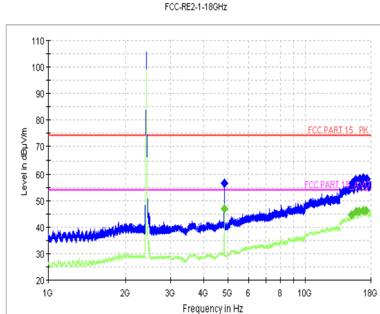
Fig.1 Radiated Spurious Emission (802.11b, Ch1, 1 GHz-18GHz)
