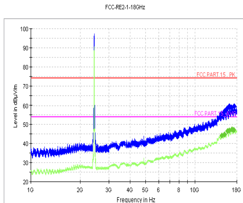
Fig.4 Radiated Spurious Emission (802.11b, Ch6, 1 GHz-18GHz)
