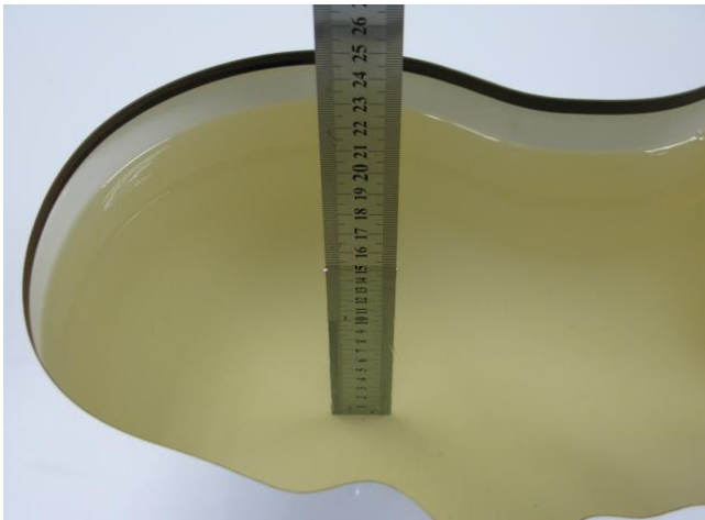
Photo 18:HSL 1750MHz depth (15.3cm)
