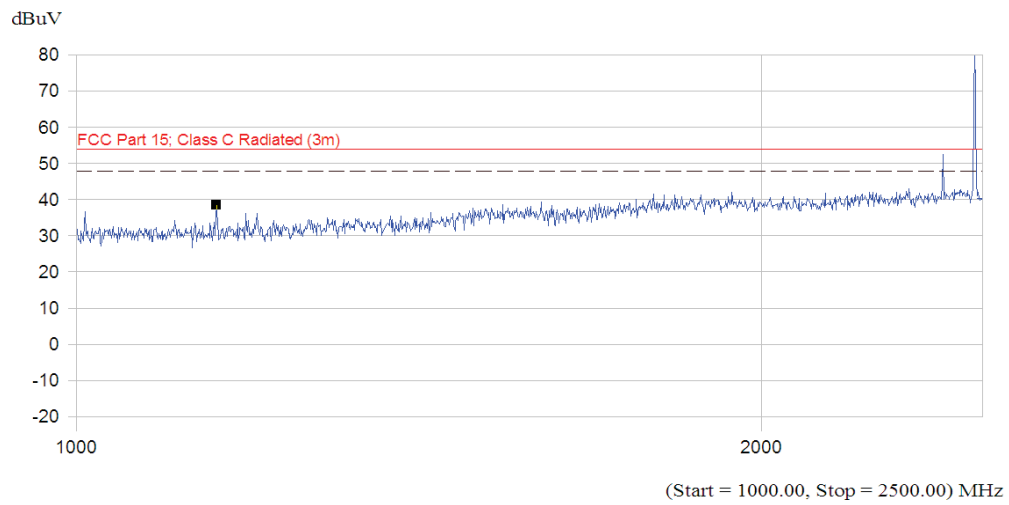
(Plot C.6: Antenna Vertical, 1GHz to 2.5GHz)
