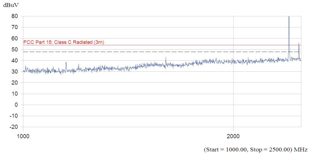
(Plot A.6: Antenna Vertical, 1GHz to 2.5GHz)
