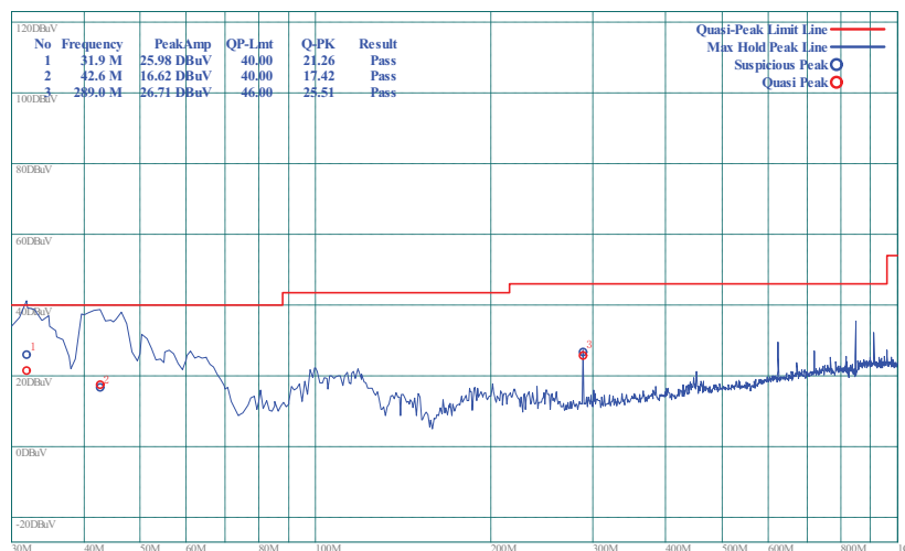
(Plot B.5: Antenna Vertical, 30MHz to 1GHz)
