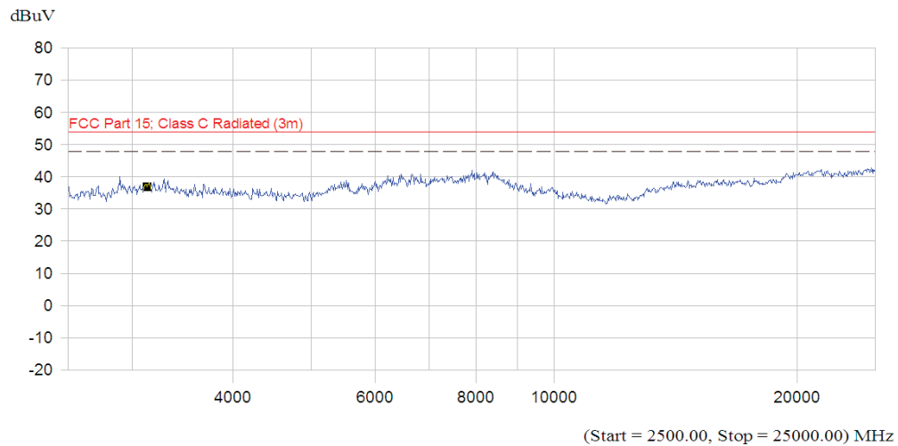
(Plot B.4: Antenna Horizontal, 2.5GHz to 25GHz)
