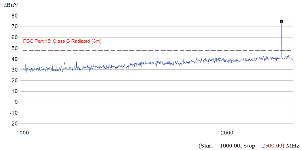
(Plot A.3: Antenna Horizontal, 1GHz to 2.5GHz)
