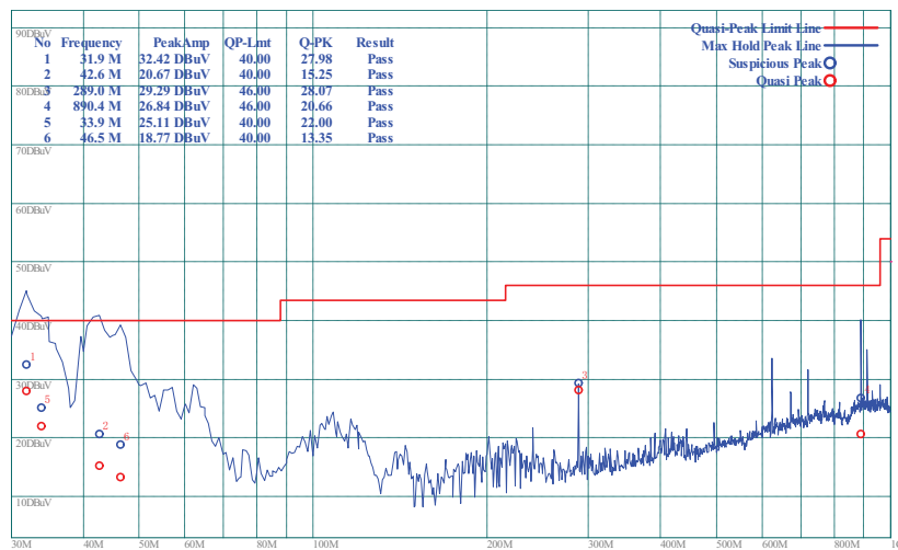
(Plot C.5: Antenna Vertical, 30MHz to 1GHz)
