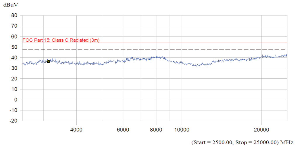
(Plot A.4: Antenna Horizontal, 2.5GHz to 25GHz)
