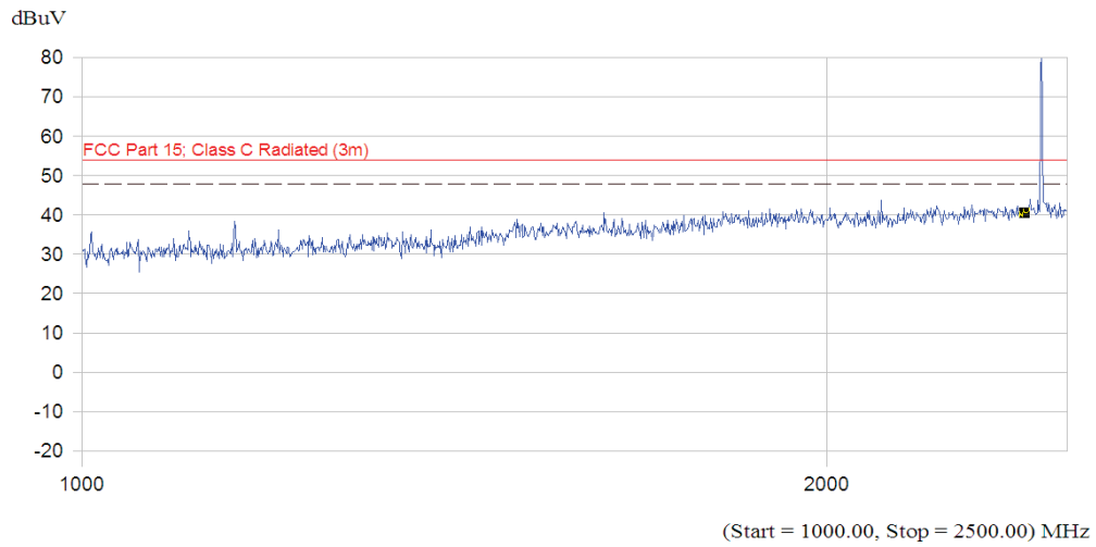
(Plot B.6: Antenna Vertical, 1GHz to 2.5GHz)
