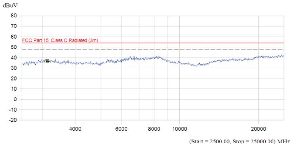
(Plot B.7: Antenna Vertical, 2.5GHz to 25GHz)
