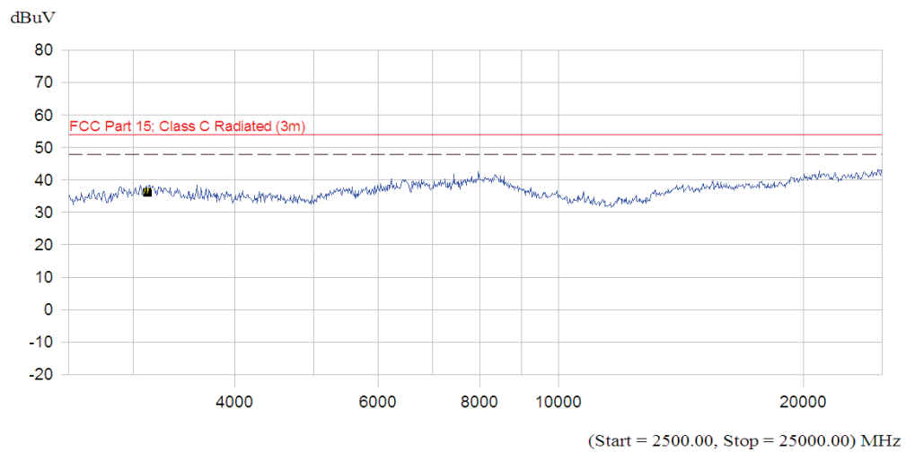
(Plot C.7: Antenna Vertical, 2.5GHz to 25GHz)
