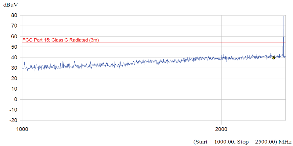
(Plot C.3: Antenna Horizontal, 1GHz to 2.5GHz)
