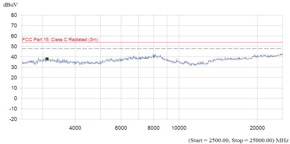
(Plot C.4: Antenna Horizontal, 2.5GHz to 25GHz)
