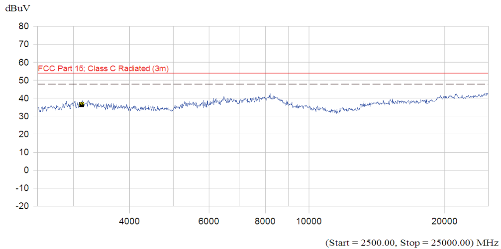
(Plot A.7: Antenna Vertical, 2.5GHz to 25GHz)
