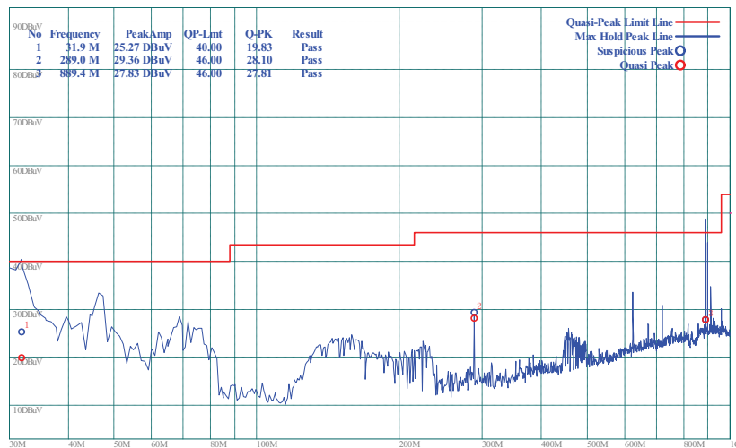
(Plot C.2: Antenna Horizontal, 30MHz to 1GHz)
