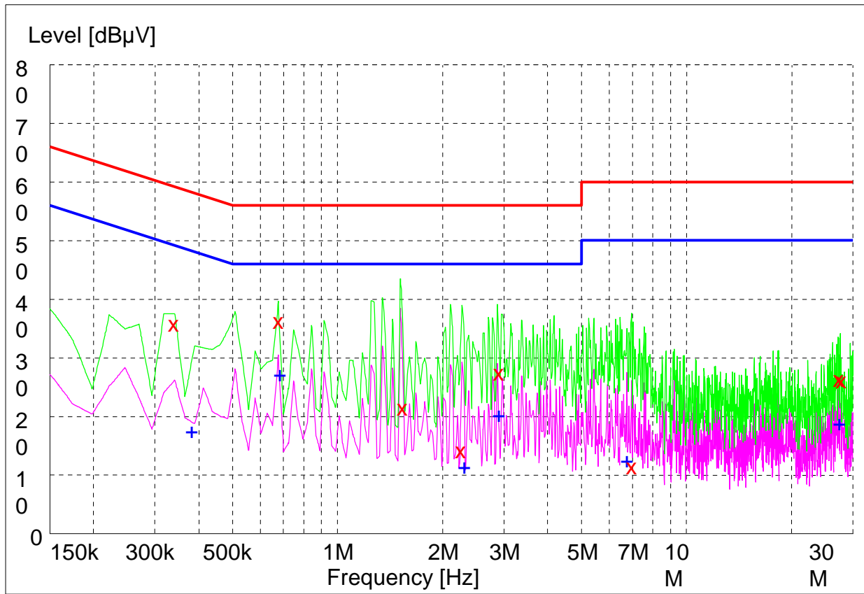
MEASUREMENT RESULT: QP Detector
