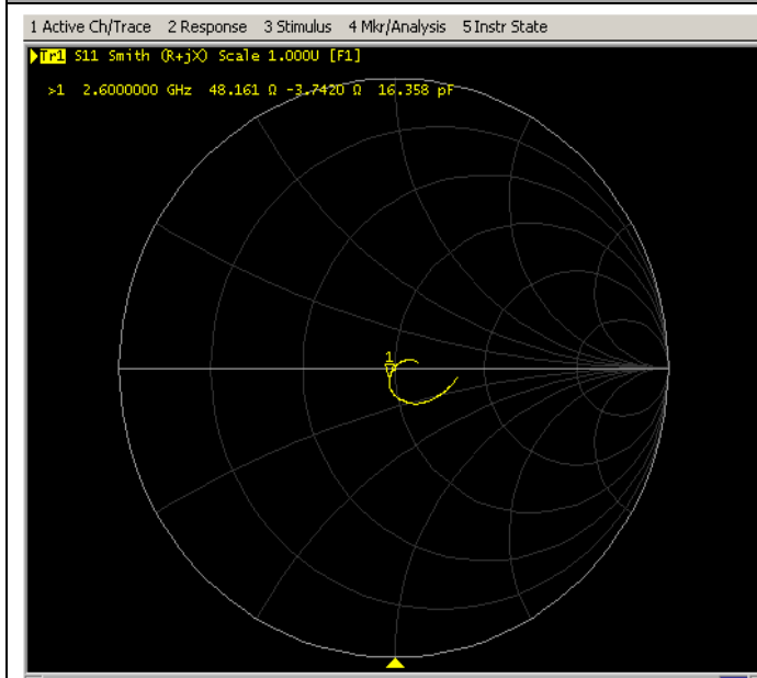
Impedance Test-Body
