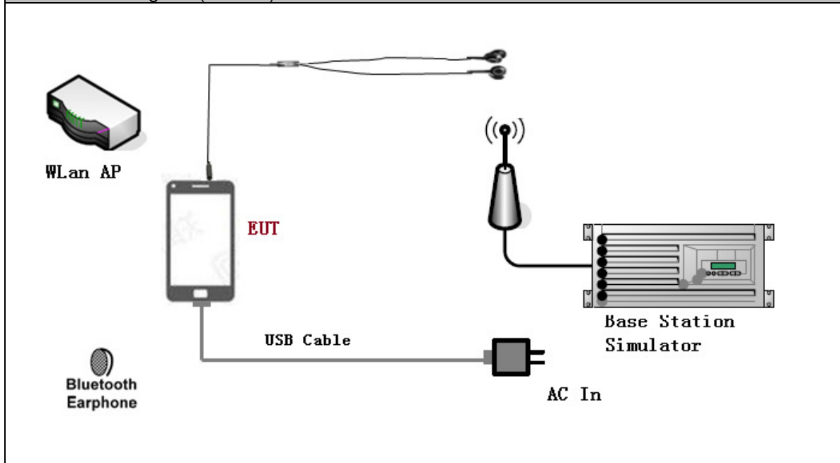
Connection Diagram (Mode 1)
