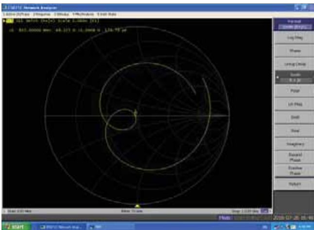
Impedance Test -Body
