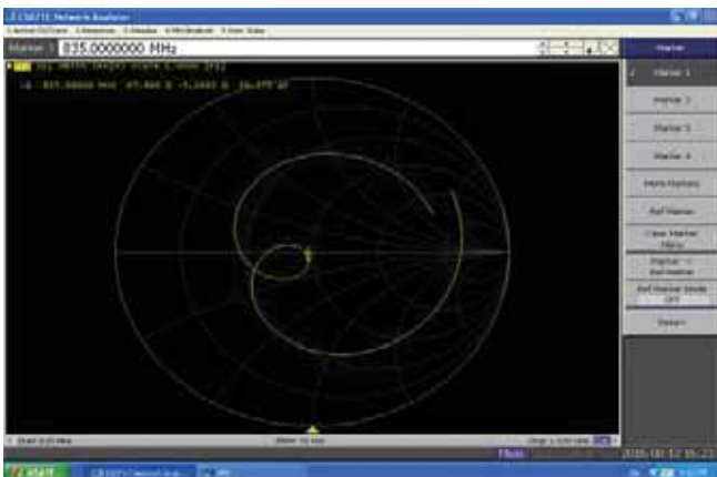
Impedance Test -Body
