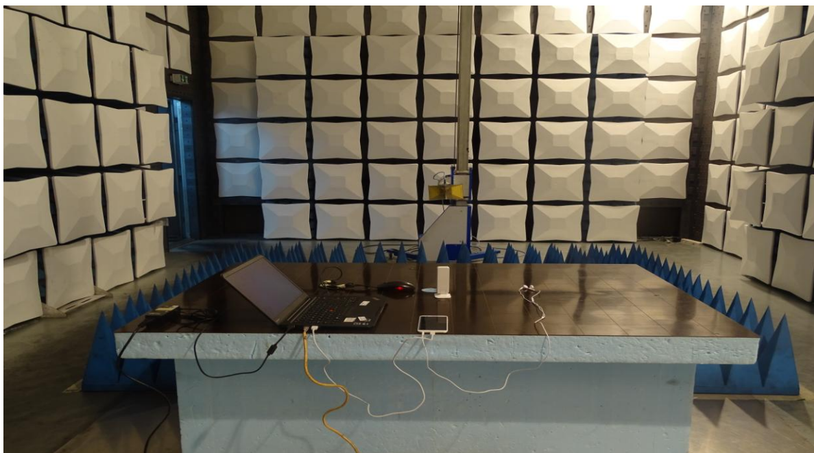
Radiated Disturbance Emissions (1GHz to18GHz)
