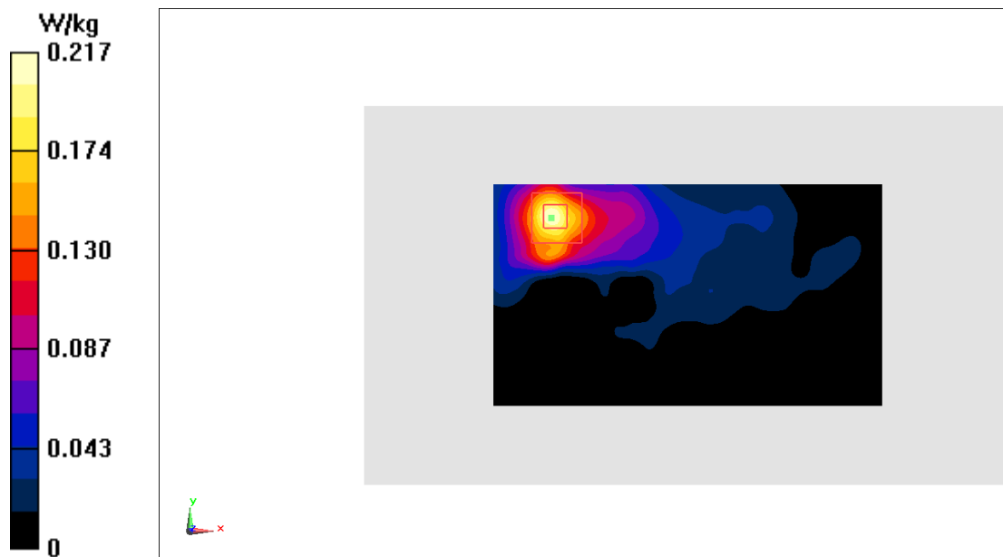
Fig.33 5GHz
