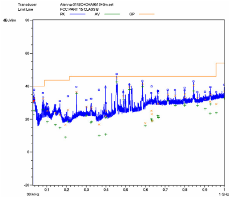
Vertical:Radiated Emission Test Plot- IP Call
