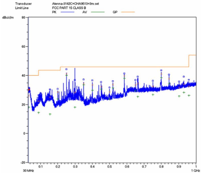
Horizontal:Radiated Emission Test Plot-IP Call
