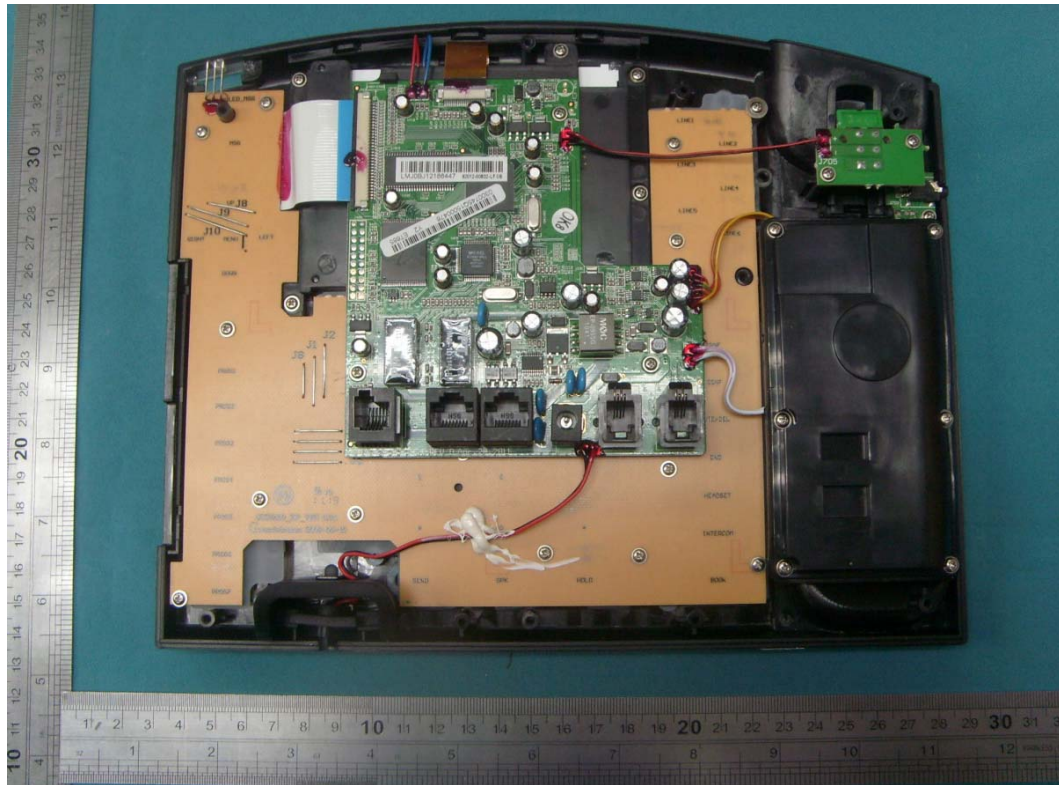
EUT-Uncovered View
