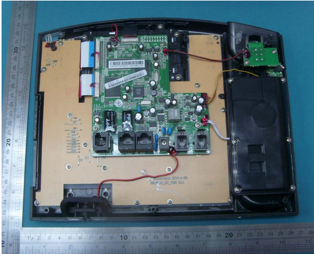
EUT-Uncovered View
