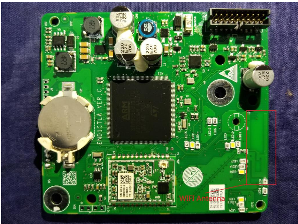
(4) EUT Photo (PCB Antenna)
