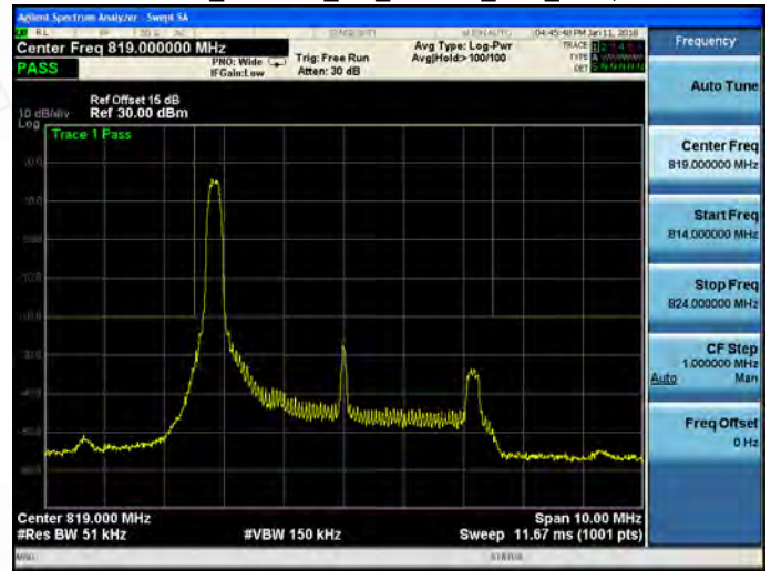
Part 90_Band 26_5M_64QAM_MID_RB1,24
