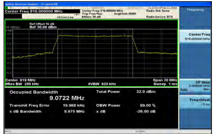
Part 90_Band26_10MHz_16QAM_50_0_MidCH26740
