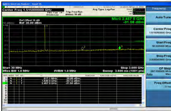
30MHz~3GHz_Band26_5MHz_QPSK_1_0_MidCH26740
