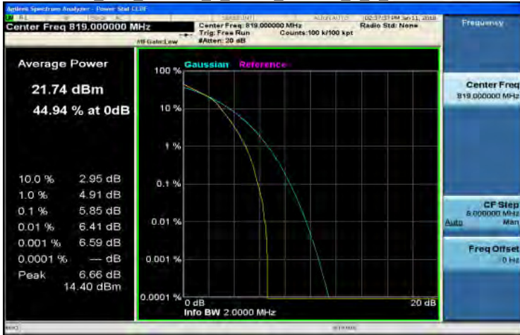
Part 90_LTE_Band26_1_4MHz_64QAM_6_0_MidCH26740
