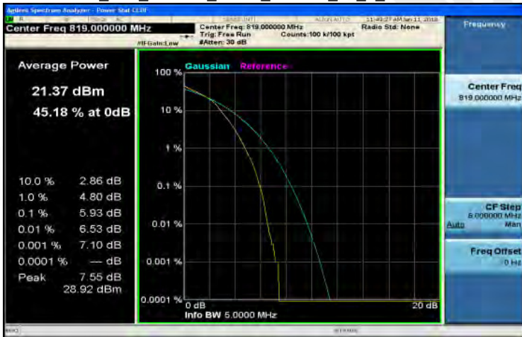
Part 90_LTE_Band26_5MHz_64QAM_25_0_MidCH26740
