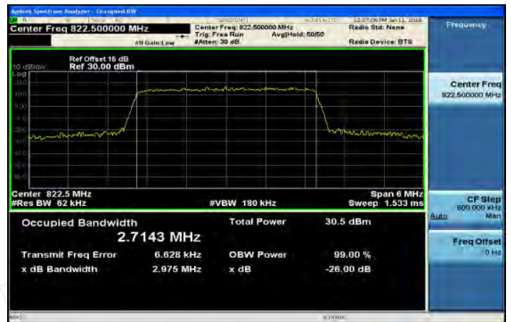
Part 90_Band26_3MHz_64QAM_15_0_HighCH26775
