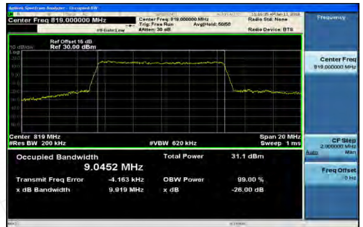
Part 90_Band26_10MHz_64QAM_50_0_MidCH26740
