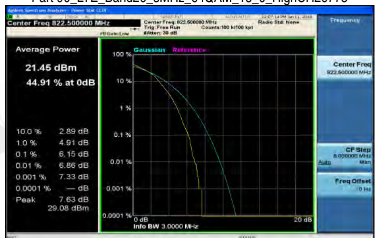
Part 90_LTE_Band26_3MHz_64QAM_15_0_HighCH26775
