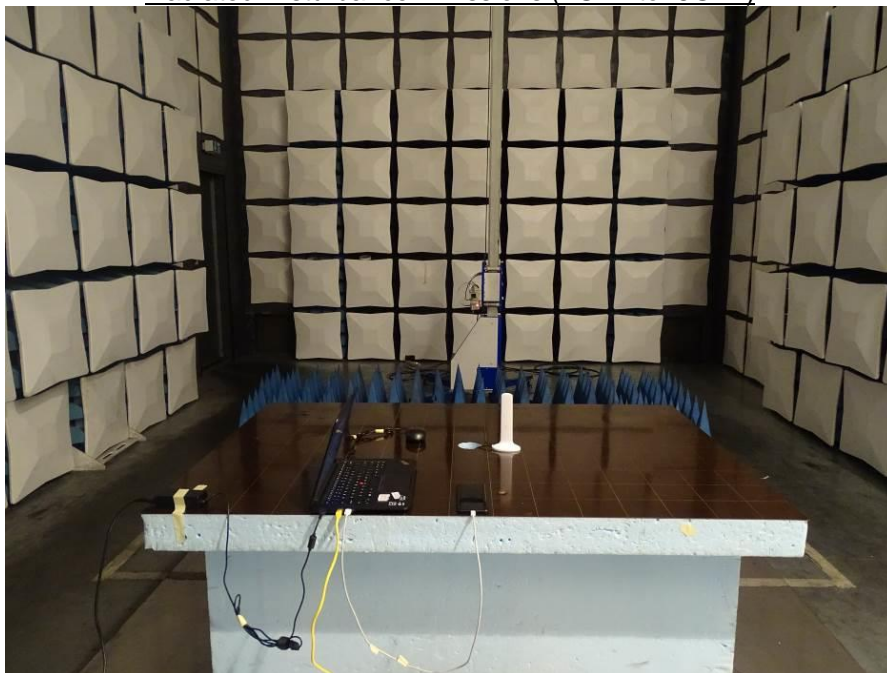
Radiated Disturbance Emissions (18GHz to 26.5GHz)
