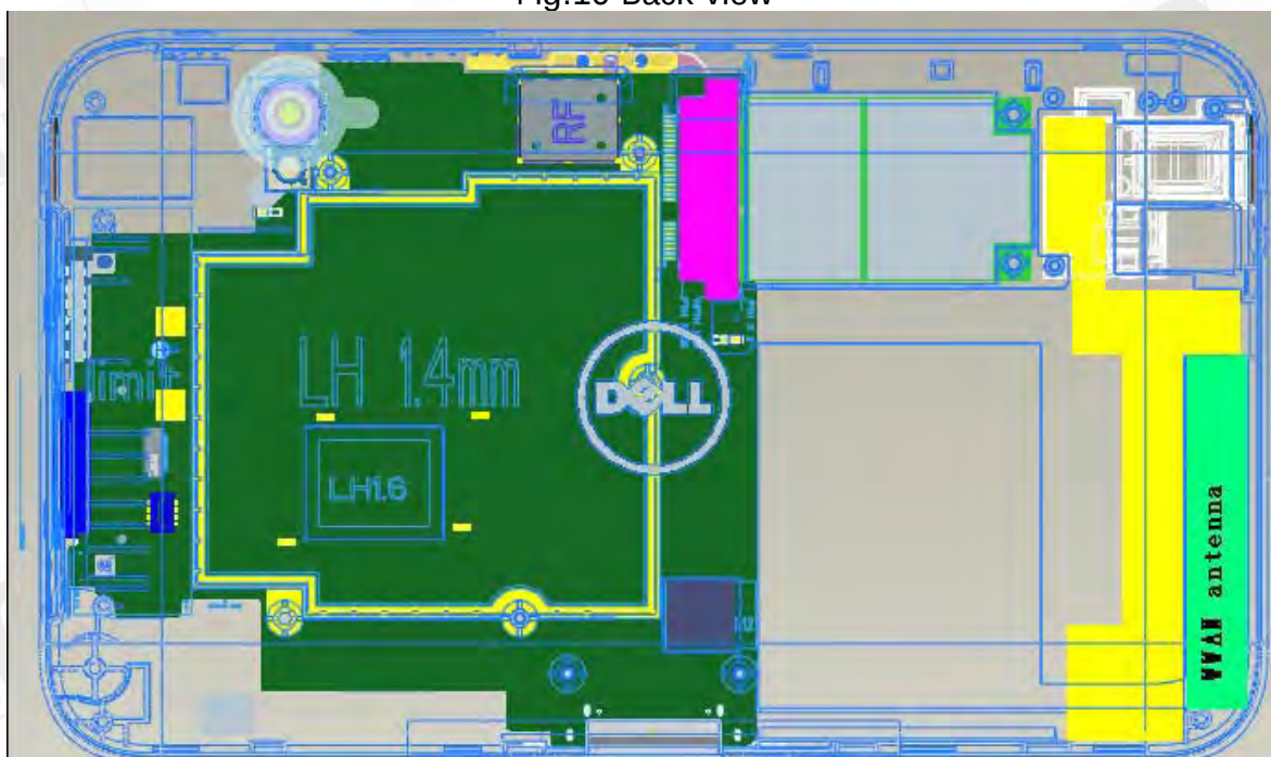
Fig.11 Proximity sensor portion in Yellow (from back view)
