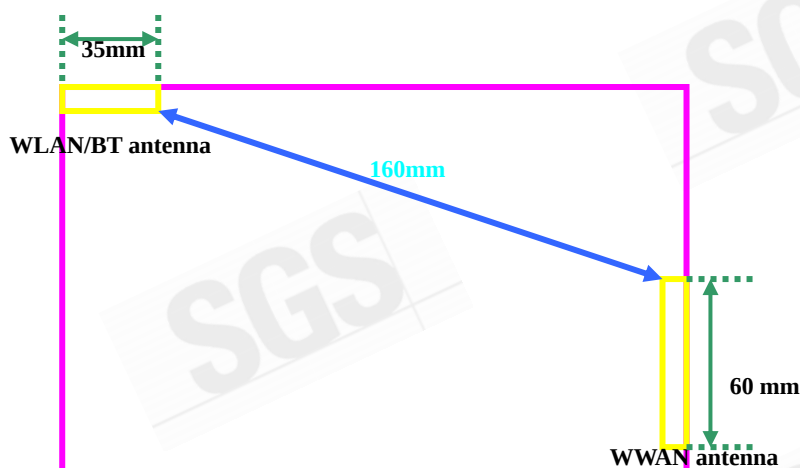
Antenna distance from Back view of EUT
