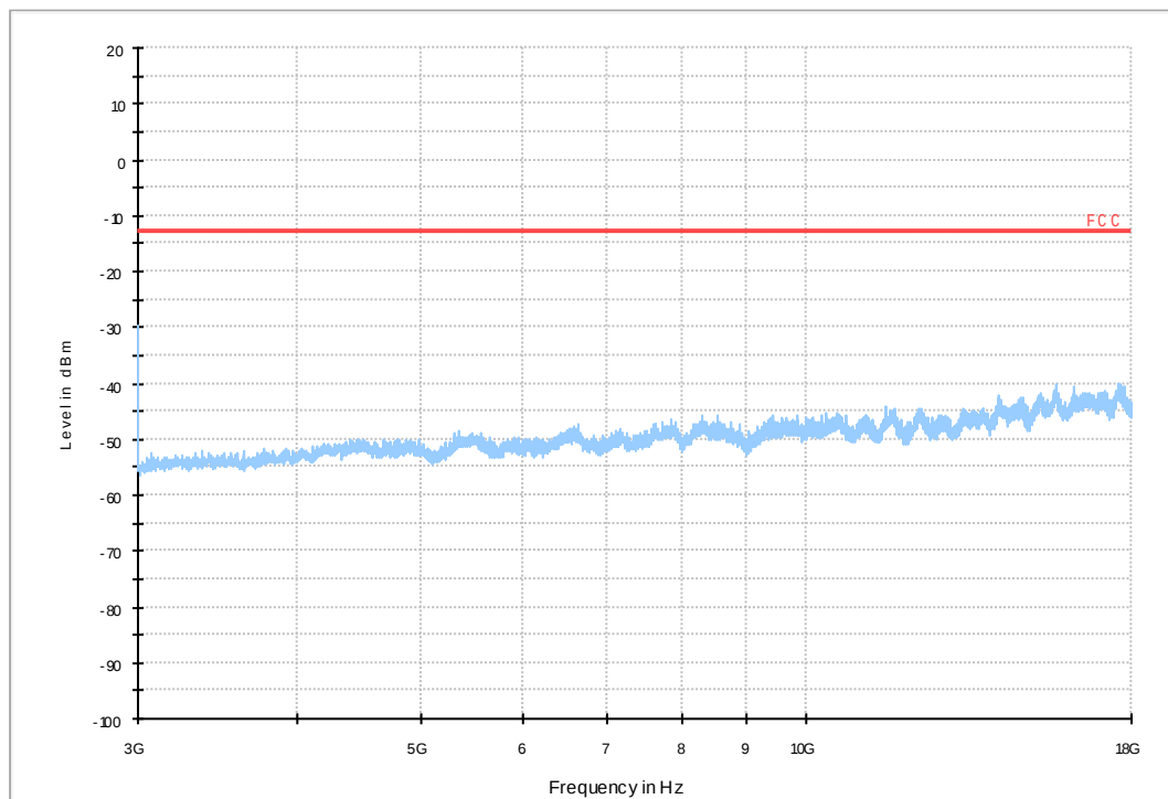
Band66/TM1_Ant2
