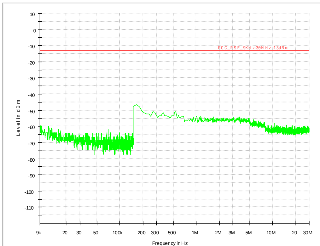
Band66/TM1_Ant2
